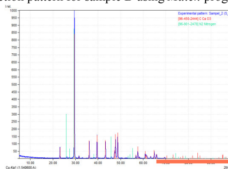
Figure 8. Difraktogram of Sample B
