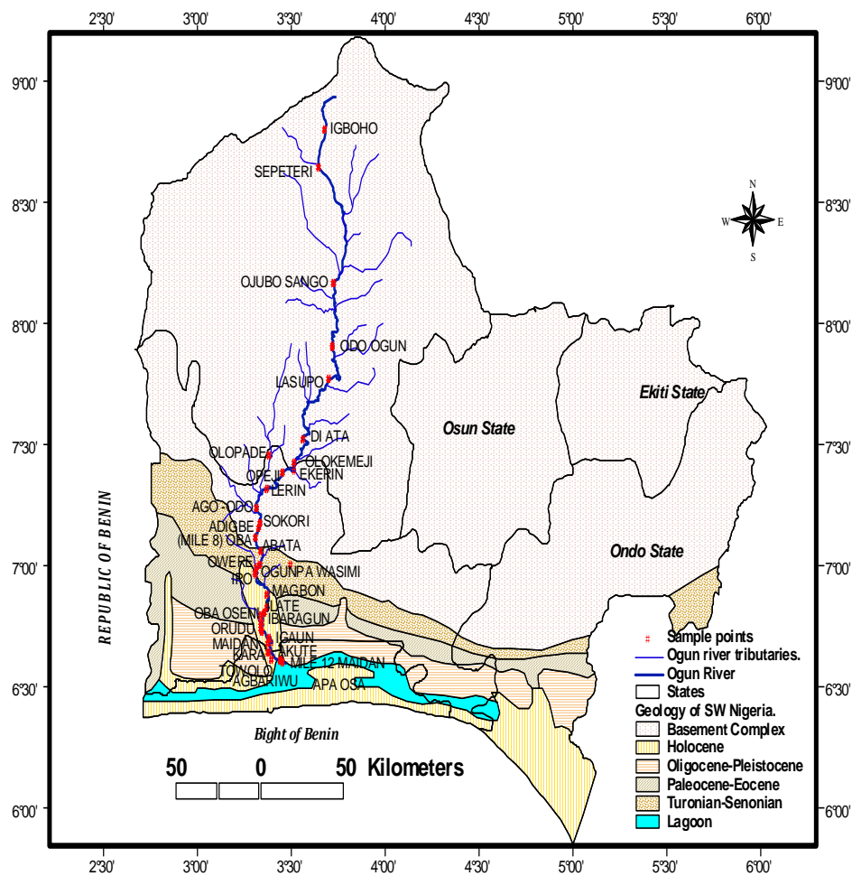
Fig. 2: The geological map of SouthWestern Nigeria showing the distribution of major sites of study (Okeyode, 2012)
