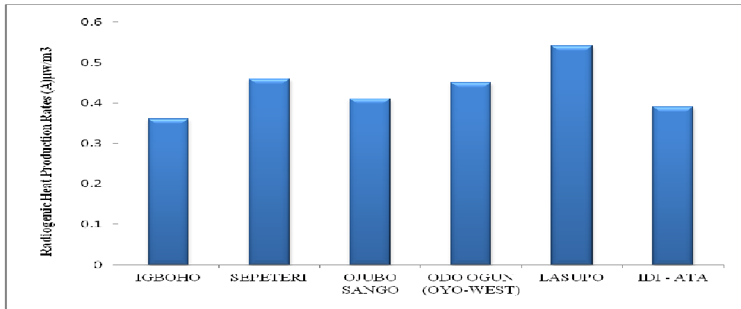
Fig. 3: Distributions of the radiogenic heat production rates for upper Ogun river
