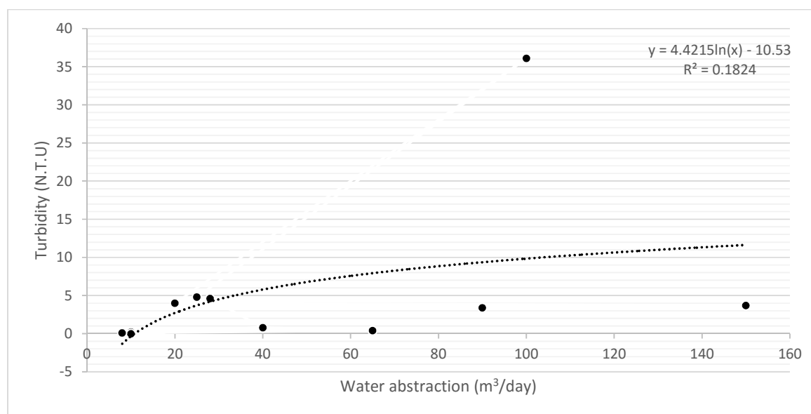
Figure 5: The relationship between groundwater turbidity and groundwater abstraction at the Yatta plateau.
