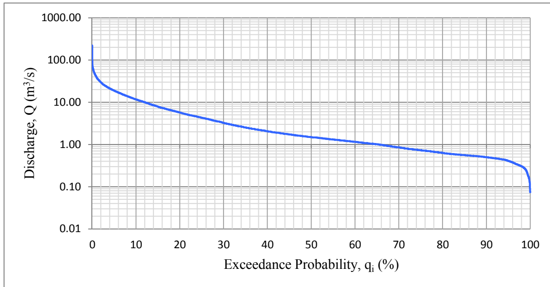
Figure 5. Daily Flow Duration Curve for the Umba River at 3KG01 Gauging Station
