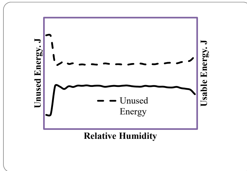
Figure 5.0 Plot of Usable and Unused Energy against Relative Humidity
