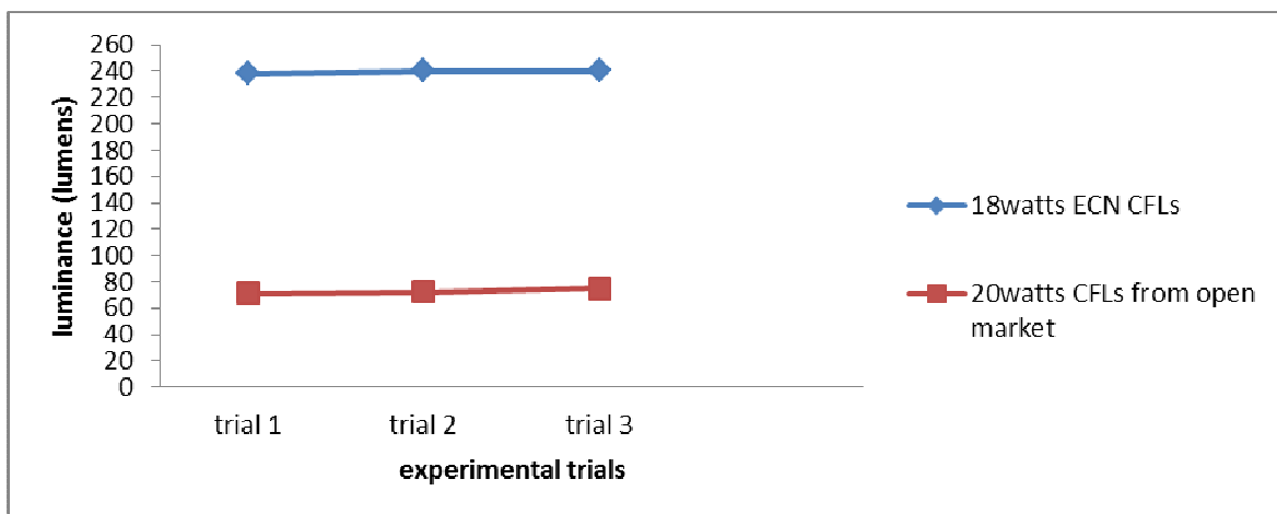
Fig 3: Results of luminance assessments for 18watts ECN CFL and 20watts CFL from open market
