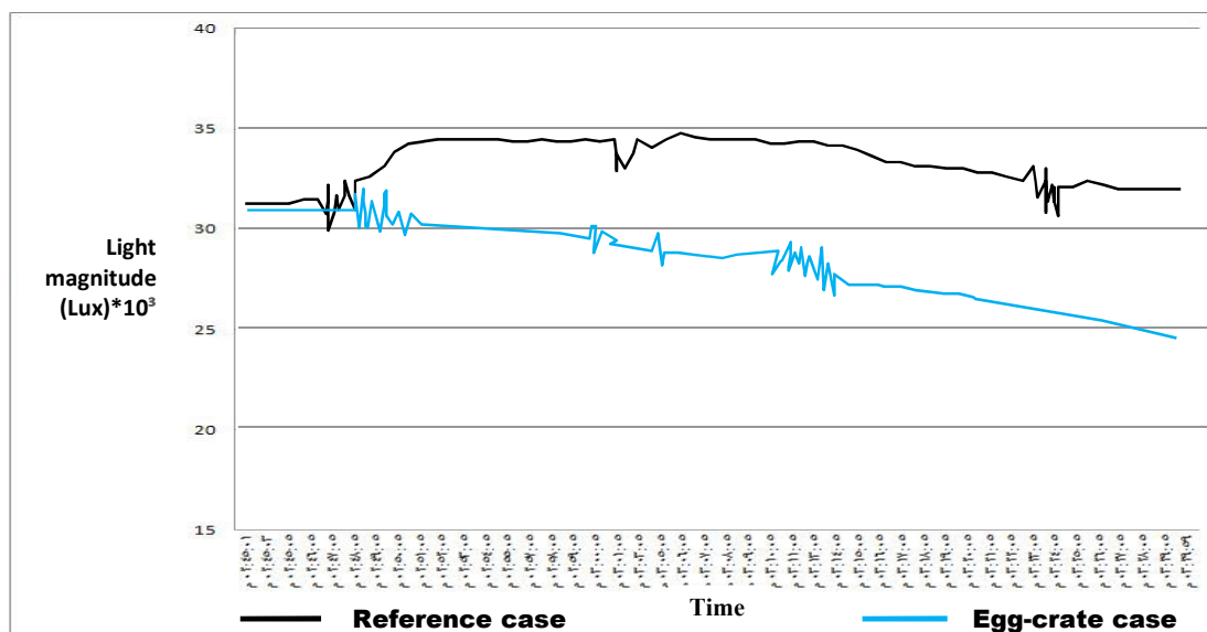
Figure 17: Egg-crate experiment result (Source:By authors).
