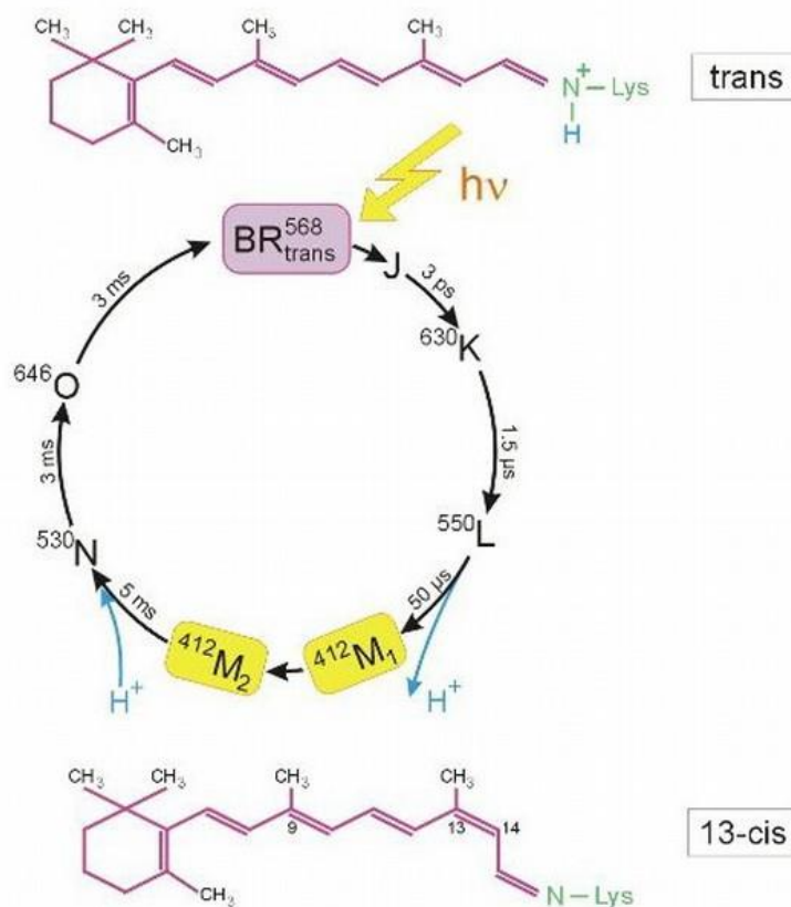
Figure 6. Photocycle scheme of BR (aqueous solution, \text{pH} = 7.2 , t = 20^\circ\text{C} ). Latin numbers J, K, L, M, N, O denote the spectral intermediates of BR. M_1 and M_2 represent spectral intermediants of meta -bacteriorhodopsin with the protonated and deprotonated aldimine bond. The superscripts correspond to the position of the absorption maximum of the photocycle intermediates (nm)
