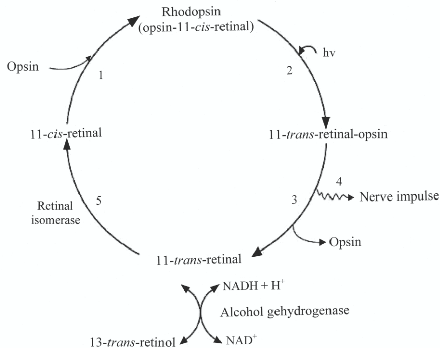
Figure 4. Photocyclus scheme of rhodopsin: 1 – 11- cis -retinal in the dark links with protein opsin to form rhodopsin; 2 – under light illumination occurs photoisomerization of 11- cis -retinal into 11- trans -retinal; 3 – 11- trans -retinal-opsin complex splits onto 11- trans -retinal and opsin; 4 – local depolarization of the membrane and the occurrence of a nerve impulse propagates along the nerve fiber; 5 – regeneration of the original pigment
