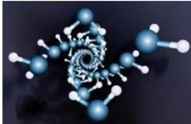
Figure 3. Structures of water crystals in carbon nanotubes according to computer simulations (Bai et al. ,
