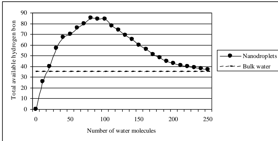
Figure 6. The total number of hydrogen bonds depending on the number of water molecules in clusters. In 2005 R. Saykally (University of California, USA) calculated the possible number of hydrogen bonds and the stability of water clusters depending on the number of H 2 O molecules (Figure 6) (Saykally, 2005). It was also estimated the possible number of hydrogen bonds (100) depending on the number of H 2 O molecules (250) in clusters (Sykes, 2007). O. Loboda and O.V. Goncharuk provided data about the existence of icosahedral water clusters consisting of 280 H 2 O molecules with the average size up to 3 nm (Loboda & Goncharuk, 2010). The ordering of water molecules into associates corresponds to a decrease in the entropy (randomness), or decrease in the overall Gibbs energy ( G = \Delta H - T\Delta S ). This means that the change in enthalpy \Delta H minus the change in entropy \Delta S (multiplied by the absolute temperature T ) is a negative value. These results are consistent with our data on research of NES spectrum of water on which it may make conclusion about the number of H 2 O molecules in water clusters. NES spectrum of water has energy ranges from -0.08 to -0.14 eV (Figure 7). The spectral range lies in the middle infrared range from 8 to 14 \mu\text{m} ("window" of the atmosphere transparency to electromagnetic radiation). Under these conditions, the relative stability of water clusters depends on external factors, primarily on the temperature.
