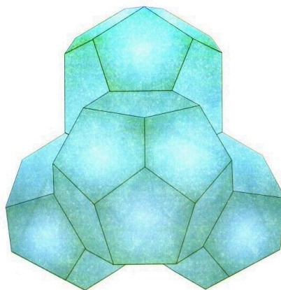
Figure 12. Model of water associate from 57 \text{H}_2\text{O} molecules. Tetrahedron of four dodecahedron ("quantum") according to the model of S. Zenin (Zenin, 1999).
