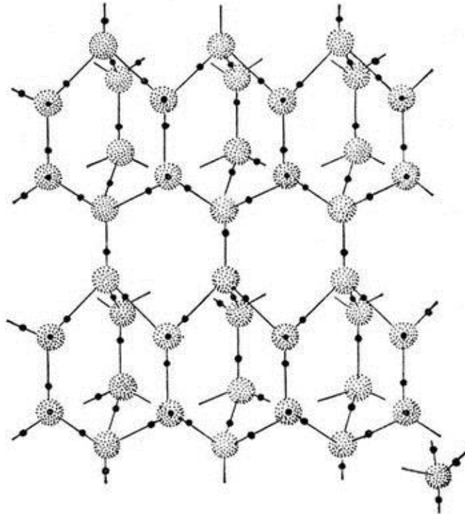
Figure 2. Hydrogen bonding in crystalline structure of natural ice \text{I}_h under the temperature -10^\circ\text{C} and pressure 1 atm. Grey balls – oxygen atoms, black balls – hydrogen atoms. On the right below shown the structural unit of crystalline ice structure.
