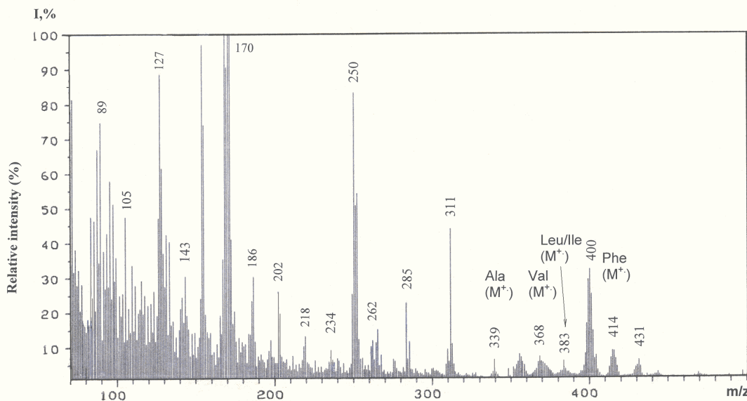
Figure 5. EI mass spectrum of methyl esters of N-DNS- [ ^2\text{H} ]amino acids from growth medium M9 containing 2% (v/v) [ ^2\text{H} ]MeOH and 49.0% (v/v) ^2\text{H}_2\text{O} (expt. 6, Table 1).
