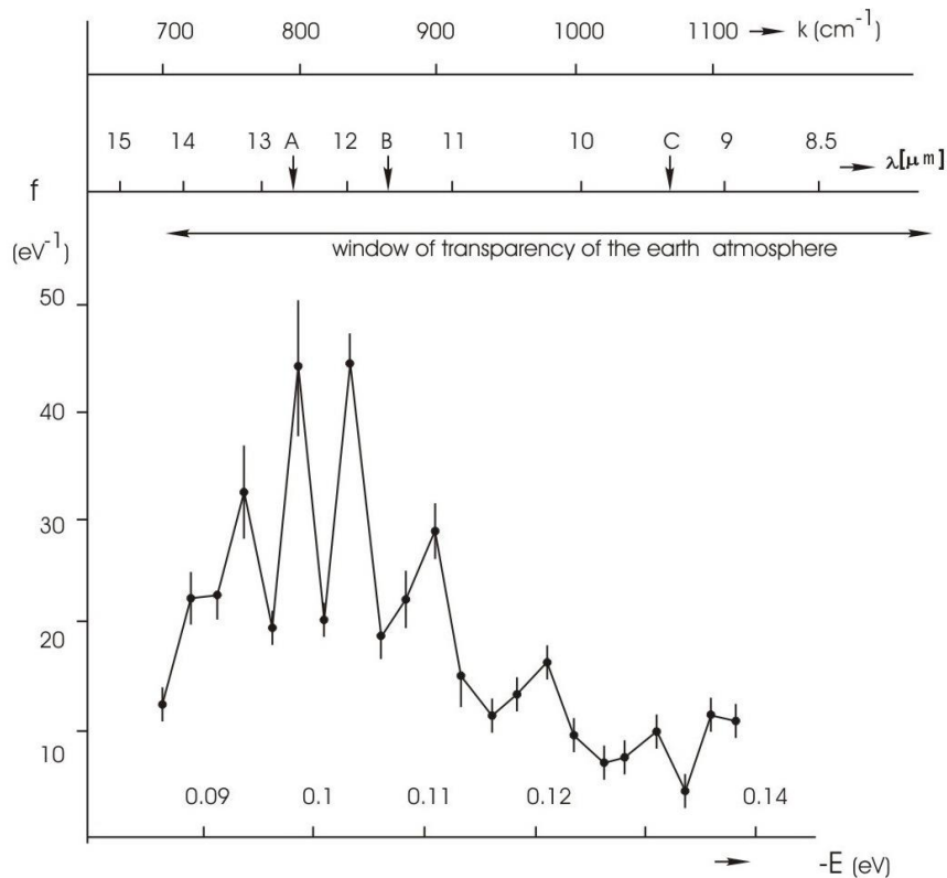
Figure 7. NES-spectrum of deionized water (chemical purity 99.99%, pH = 6.5–7.5, total mineralization 200 mg/l, electric conductivity 10 \mu\text{S/cm} ). On the horizontal axis shows the energy of the H...O hydrogen bonds in the associates -E (eV). The vertical axis – energy distribution function -f ( \text{eV}^{-1} ). k – the vibration
