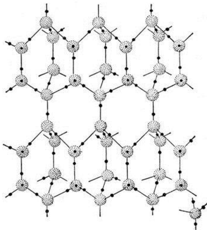
Figure 2. Hydrogen bonding in crystalline structure of natural ice I_h under the temperature -10^{\circ}C and pressure 1 atm. Grey balls – oxygen atoms, black balls – hydrogen atoms. On the right below shown the structural unit of crystalline ice structure.
