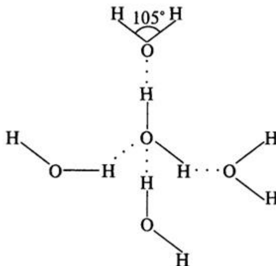
Figure 1. Hydrogen bonding between four individual H 2 O molecules. It is shown the value of the angle between the covalent H–O–H bond in H 2 O molecule.
