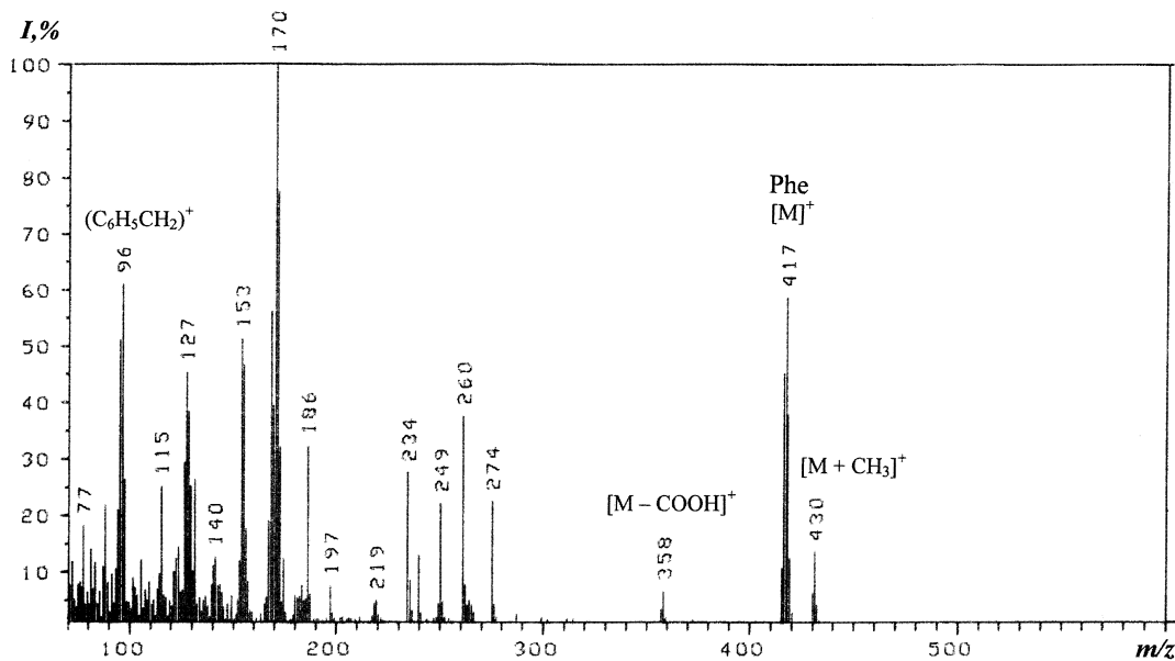
Figure 4. EI mass spectra of methyl N-Dns-[2,3,4,5,6- ^2\text{H}_5 ]Phe under various experimental conditions: a) – the unlabeled methyl ester of N-Dns-Phe; b) – methyl ester of N-Dns-[2,3,4,5,6- ^2\text{H}_5 ]Phe, isolated from the BR hydrolyzate by RP HPLC. Separation conditions: 250 × 10 mm Column C18 (“Kova”, Slovakia), eluents: (A) – \text{CH}_3\text{CN}-\text{CF}_3\text{COOH} (100: 0.1–0.5% (v/v)) and (B) – \text{CH}_3\text{CN} (100% (v/v)).
