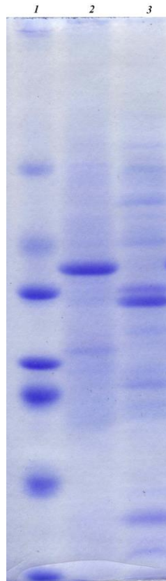
Figure. 5. Electropherograms of proteins isolated from hydrolysates of total biomass of B. subtilis : 1 – a standard set of proteins; 2 – a sample obtained from protonated medium; 3 – a sample obtained from D 2 O-medium
