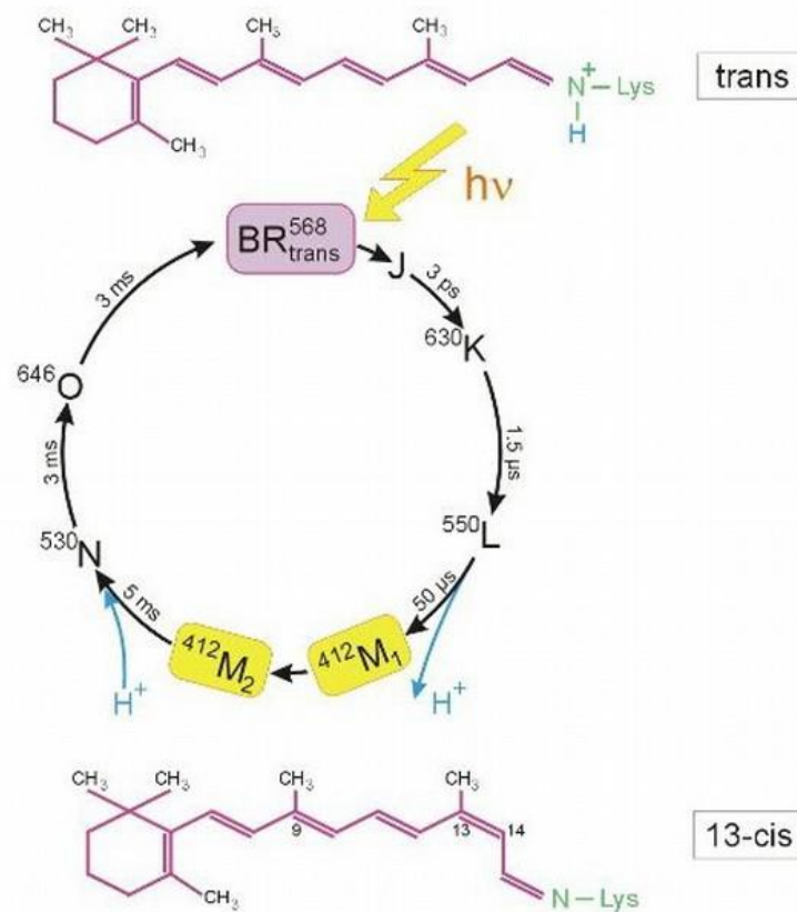
Figure 6. Photocycle scheme of BR (aqueous solution, pH = 7.2, t = 20^\circ\text{C} ). Latin numbers J, K, L, M, N, O denote the spectral intermediates of BR. M 1 and M 2 represent spectral intermediants of meta -bacteriorhodopsin with the protonated and deprotonated aldimine bond. The superscripts correspond to the position of the absorption maximum of the photocycle intermediates (nm)
