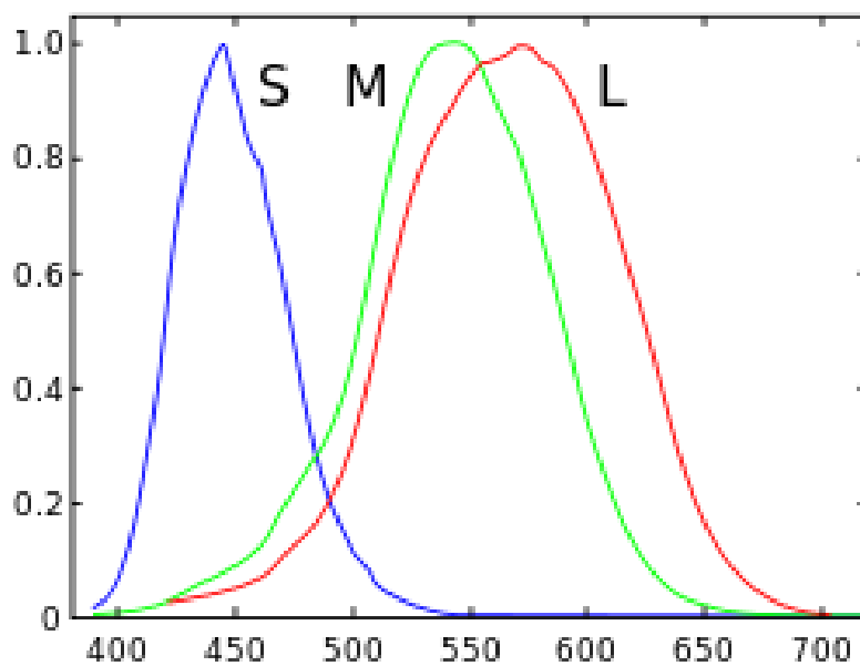
Figure 8. Spectral sensitivity of the different types of receptor cells (cones) in the retina
