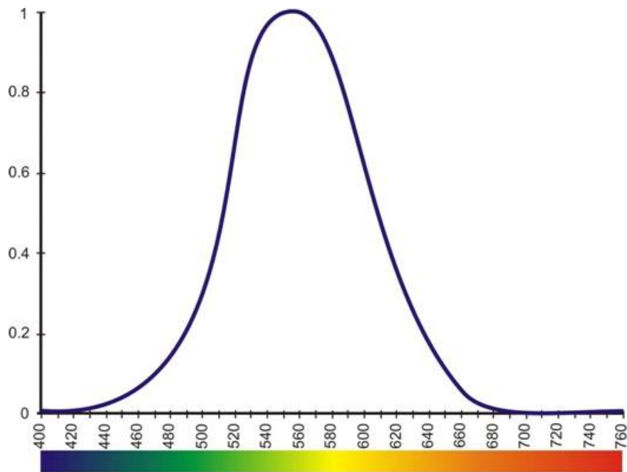
Figure 9. Spectral sensitivity of the visual analyzer
