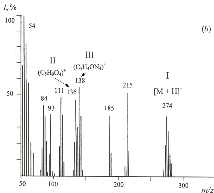
Figure 4. FAB mass spectra of inosine (glycerol as a matrix) under different experimental conditions: (a) – natural inosine; (b) – [^2\text{H}] inosine isolated from HW medium (scanning interval at m/z 50–350; major peaks with a relative intensity of 100% at m/z 52 and m/z 54; ionization conditions: cesium source; accelerating voltage, 5 kV; ion current, 0.6–0.8 mA; resolution, 7500 arbitrary units): I – relative intensity of peaks (%); (I) – inosine; (II) – ribose fragment; (III) – hypoxanthine fragment.
