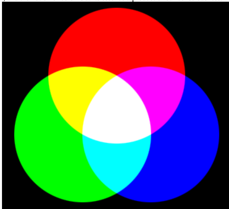
Figure 10. Additive mixing of colors
