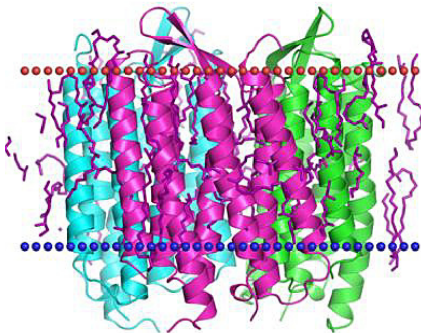
Figure 5. The structure of BR from PM of halophilic bacterium H. halobium according to computer modeling data
