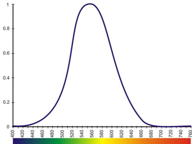
Figure 9. Spectral sensitivity of the visual analyzer
