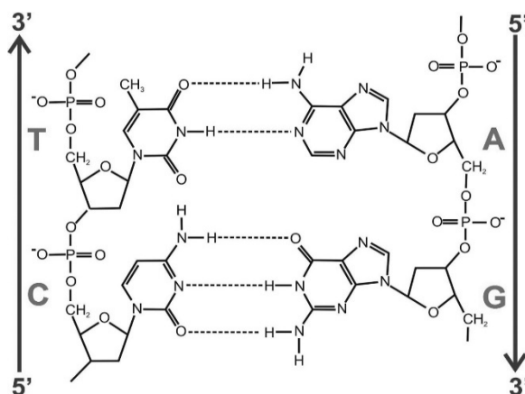
Figure 1a Hydrogen bonds among H and N or O in DNA
