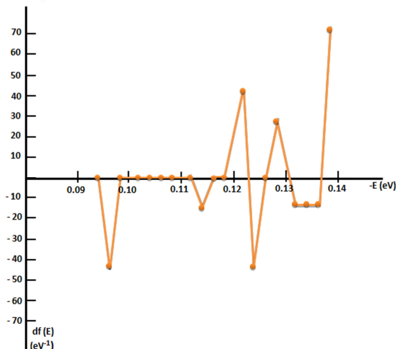
Figure 4. DNES of 1% solution of blood serum of hamsters with tumors with influence of e.m. fields as difference from the control group of hamsters with tumors.
