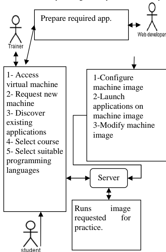
Figure 6. Processes of the Proposed Solution .
