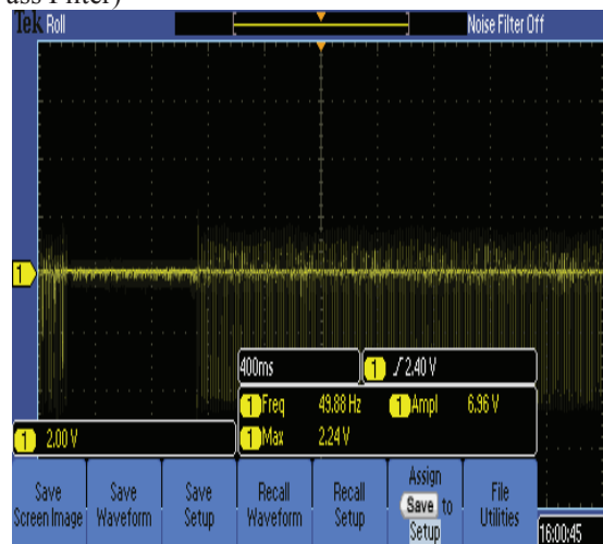
Figure 8 Output of LPF
