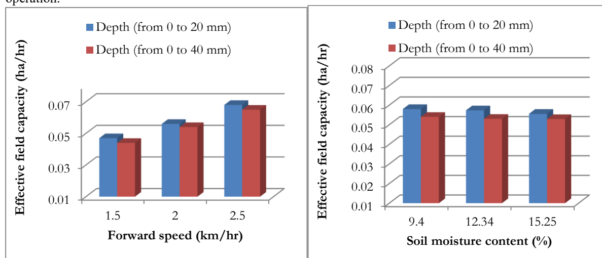
Figure 4. Effect of soil moisture and machine operational parameter on effective field capacity
