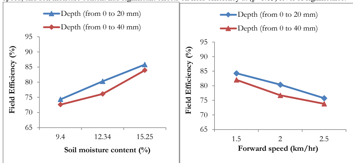
Figure 5: Effect of soil moisture and machine operational parameters on the field efficiency
