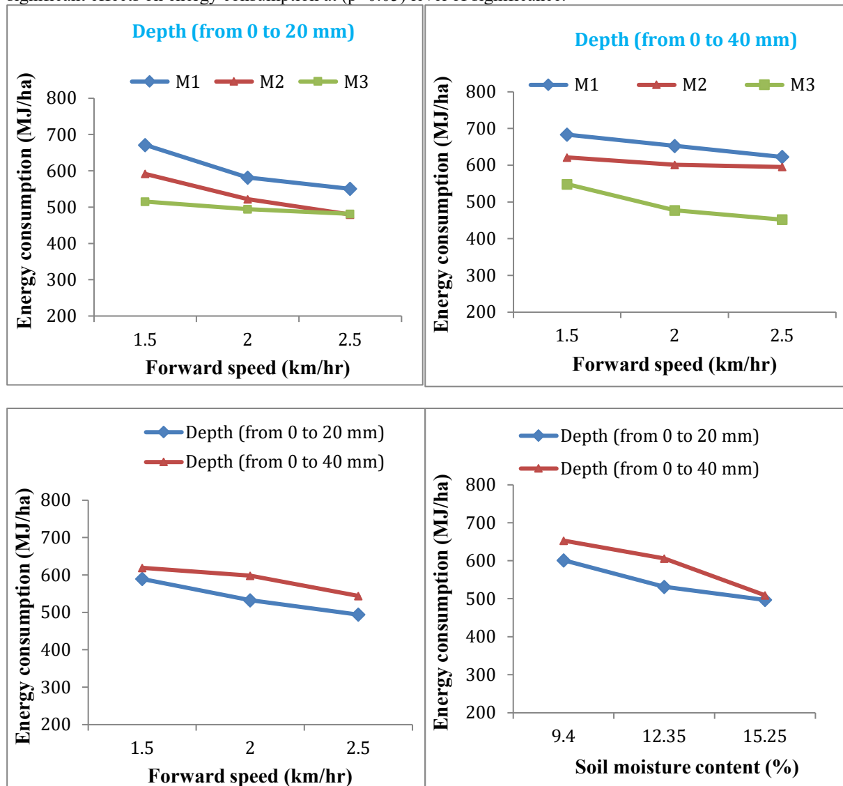
Figure 8: Effect of soil moisture and machine operational parameters on energy consumption
