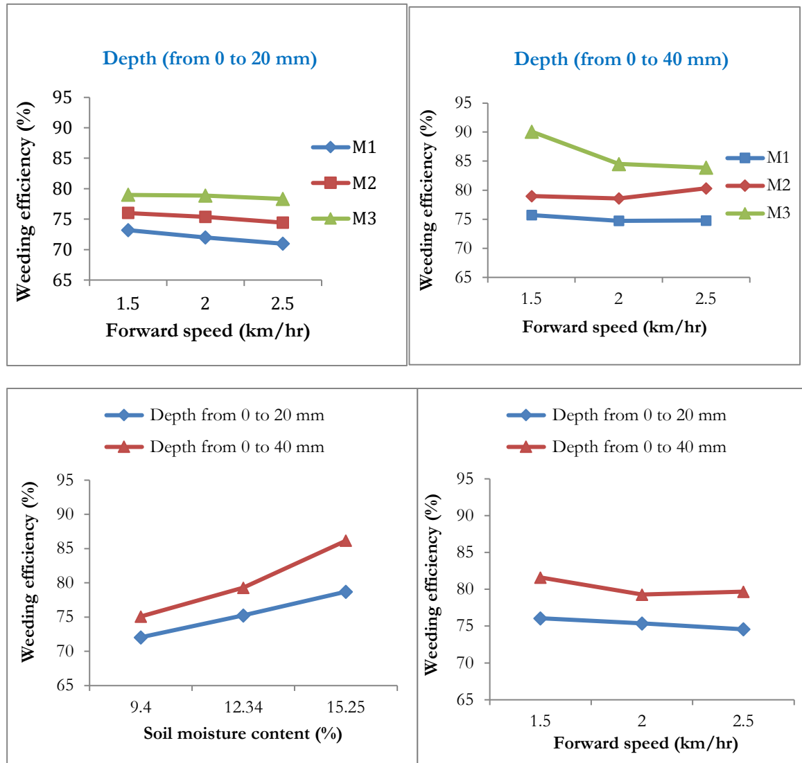
Figure 2: Effect of soil moisture and machine operational parameter weeding efficiency
