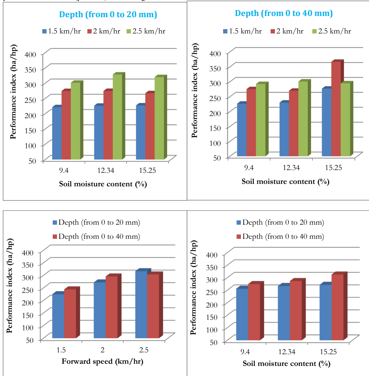
Figure 7: Effect of soil moisture and machine operational parameters on a performance index
