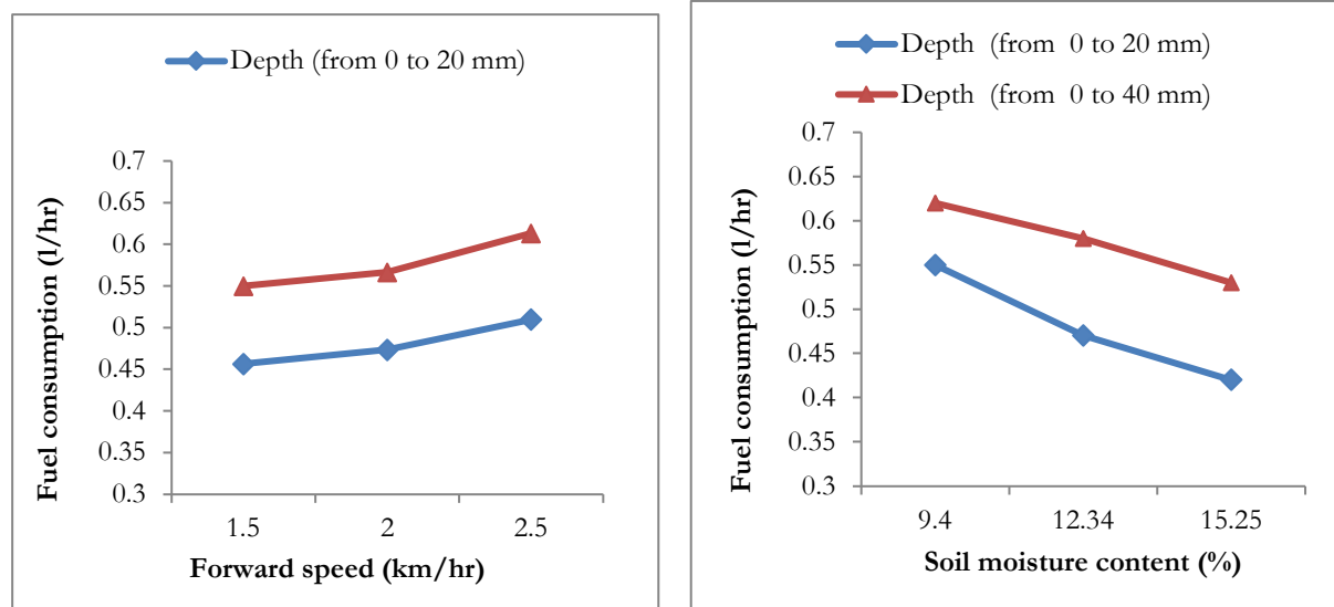
Figure 6: Effect of soil moisture and machine operation parameter on fuel consumption
