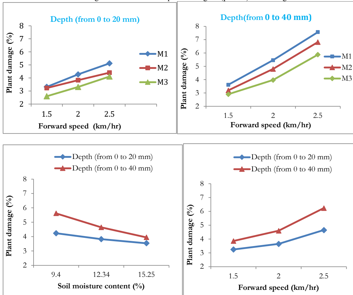
Figure 3: Effect of soil moisture and machine operational parameters on plant damage
