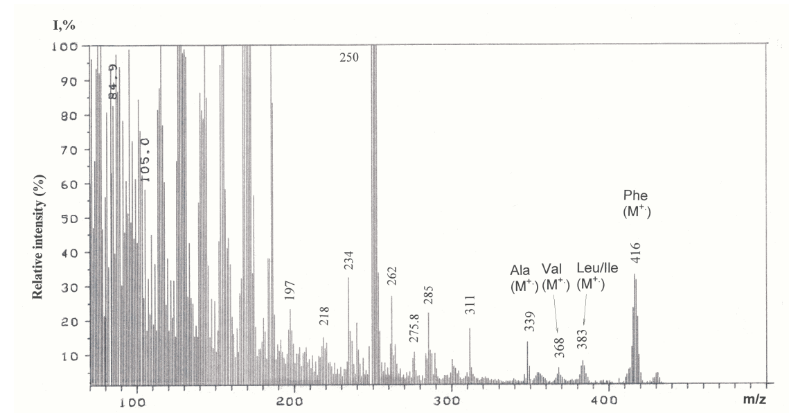
Figure 6. EI mass spectrum of methyl esters of N-DNS-[ 2 H]amino acids from growth medium M9 containing 2% (v/v) [U- 2 H]MeOH and 73.5% (v/v) 2 H 2 O (expt. 8, Table 1).
