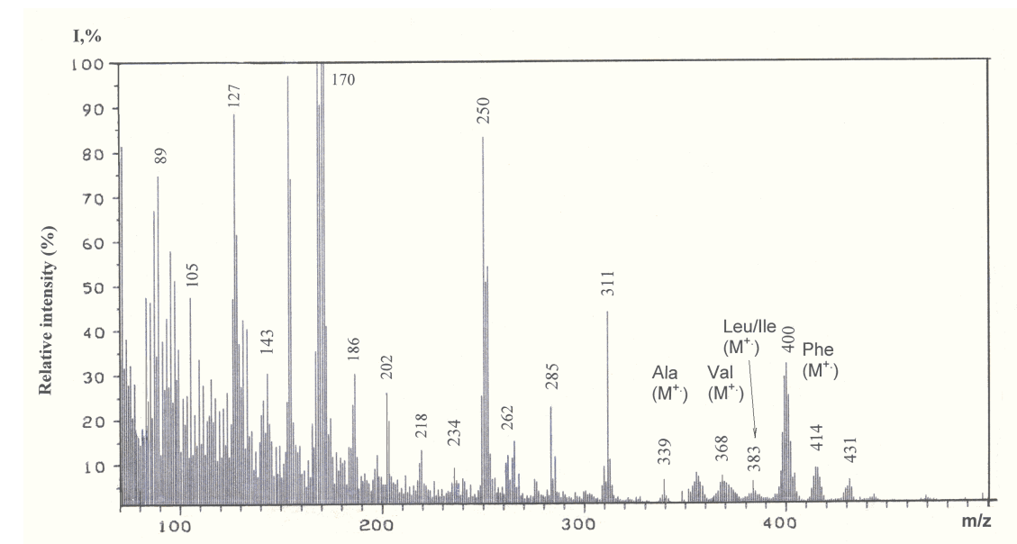
Figure 5. EI mass spectrum of methyl esters of N-DNS- [^2H] amino acids from growth medium M9 containing 2% (v/v) [ U - ^2H ]MeOH and 49.0% (v/v) ^2H_2O (expt. 6, Table 1).
