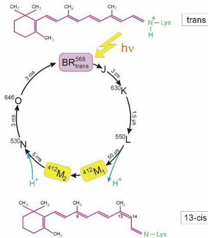
Figure 6. Photocycle scheme of BR (aqueous solution, \text{pH} = 7.2 , t = 20 \text{ }^{\circ}\text{C} ). Latin numbers J, K, L, M, N, O denote the spectral intermediates of BR. \text{M}_1 and \text{M}_2 represent spectral intermediants of meta -bacteriorhodopsin with the protonated and deprotonated aldimine bond. The superscripts correspond to the position of the absorption maximum of the photocycle intermediates (nm)
