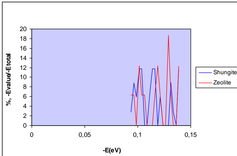
Figure 4. The distribution ( \% , (-E_{value})/(-E_{total}) ) of water molecules in water solution of shungite/zeolite according to energies of hydrogen bonds ( -E_{value} ) to total result of hydrogen bonds energy
