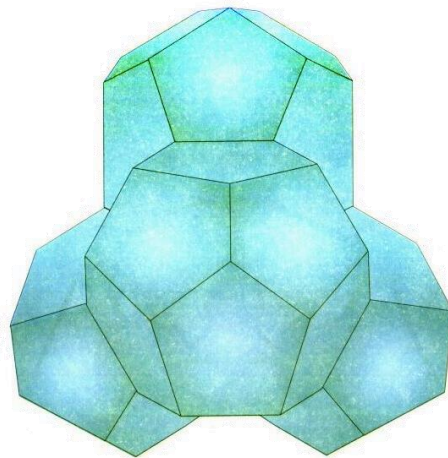
Figure 11. Model of water associate from 57 H 2 O molecules. Tetrahedron of four dodecahedron (“quantum”) according to the model of S. Zenin (Zenin, 1999).
