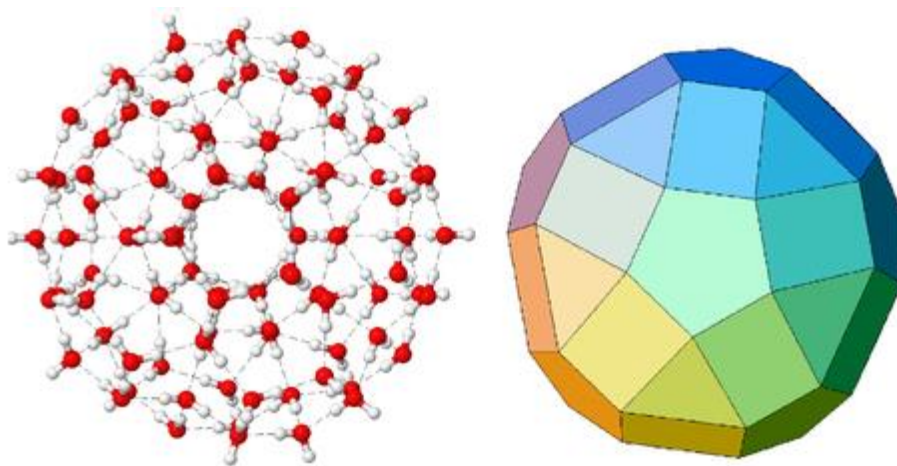
Figure 12. Icosahedron cluster based on 100 H 2 O molecules and the underlying structure.
