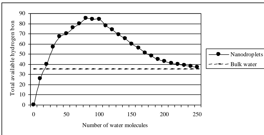
Figure 6. The total number of hydrogen bonds depending on the number of water molecules in clusters. In 2005 R. Saykally (University of California, USA) calculated the possible number of hydrogen bonds and
