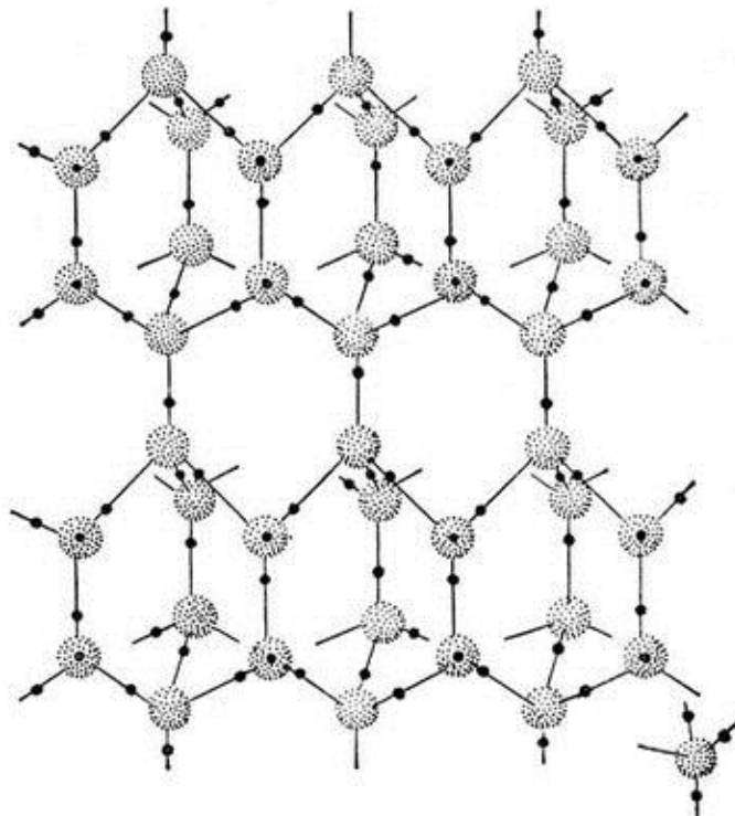
Figure 2. Hydrogen bonding in crystalline structure of natural ice I h under the temperature -10°C and pressure 1 atm. Grey balls – oxygen atoms, black balls – hydrogen atoms. On the right below shown the structural unit of crystalline ice structure.
