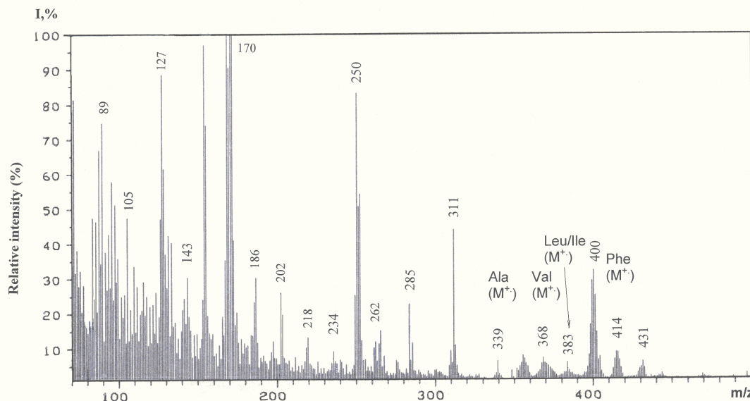
Figure 5. EI mass spectrum of methyl esters of N-DNS- [ ^2\text{H} ]amino acids from growth medium M9 containing 2% (v/v) [ ^2\text{H} ]MeOH and 49.0% (v/v) ^2\text{H}_2\text{O} (expt. 6, Table 1).
