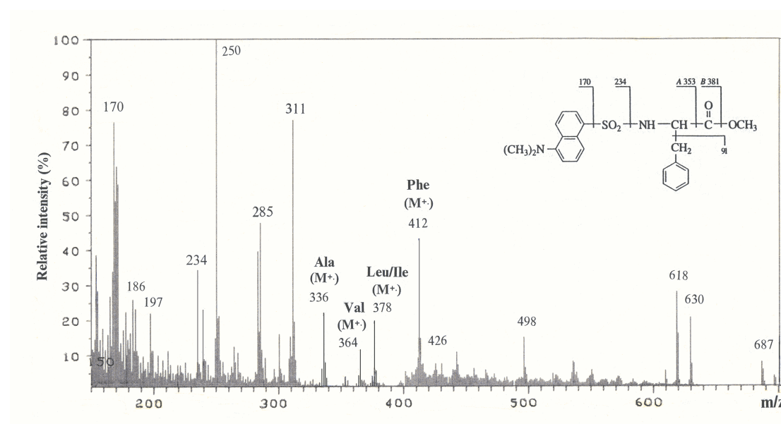
Figure 4. EI Mass spectrum of methyl esters of N-DNS-amino acids from protonated growth medium M9 (expt. 1, Table 1) after processing by DNSCl and DZM, and fragmentation of methyl ester of N-DNS-phenylalanine by EI MS method. Symbols of amino acids refer to the peaks of molecular ions ( M^+ ) of methyl esters of N-DNS-amino acids.
