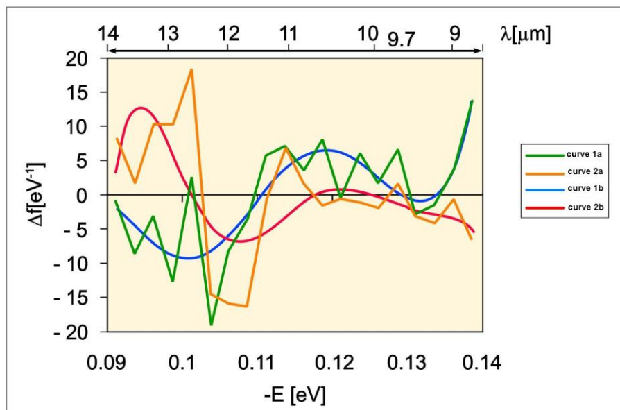
Fig. 4. Differential non-equilibrium energy spectrum (DNES) reflecting the heat exchange of the human body with the surrounding environment.
