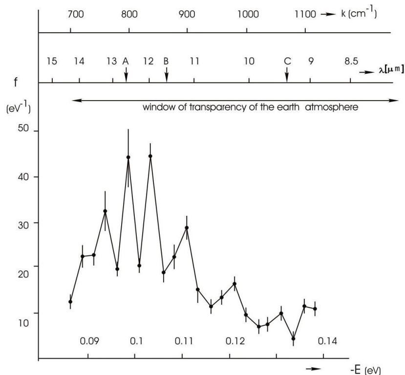
Fig. 3. Non-equilibrium energy spectrum (NES) of water as a result of measurement for 1 year: \lambda – wavelength, k – wave number.
