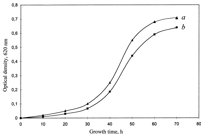
Figure 1. Growth dynamics of H. halobium under various experimental conditions: a) – protonated synthetic medium; b) – synthetic medium with [2,3,4,5,6- ^2\text{H}_5 ]Phe (0.26 g/l), [3,5- ^2\text{H}_2 ]Tyr (0.2 g/l) and [2,4,5,6,7- ^2\text{H}_5 ]Trp (0.5 g/l). The incubation period: 4–5 days, temperature: 35 °C, illumination under monochrome light at \lambda = 560 nm.
