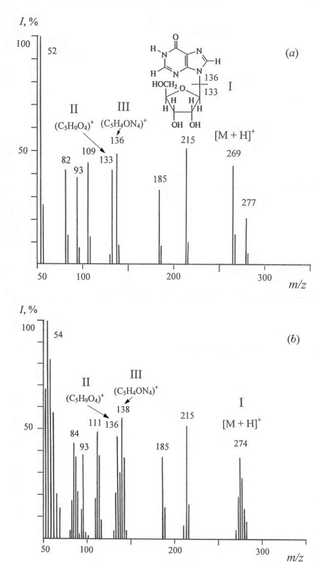
Figure 5. FAB mass spectra of inosine (glycerol as a matrix) under different experimental conditions: (a) – natural inosine; (b) – [^2\text{H}] inosine isolated from HW medium (scanning interval at m/z 50–350; major peaks with a relative intensity of 100% at m/z 52 and m/z 54; ionization conditions: cesium source; accelerating voltage, 5 kV; ion current, 0.6–0.8 mA; resolution, 7500 arbitrary units): I – relative intensity of peaks (%); (I) – inosine; (II) – ribose fragment; (III) – hypoxanthine fragment.
