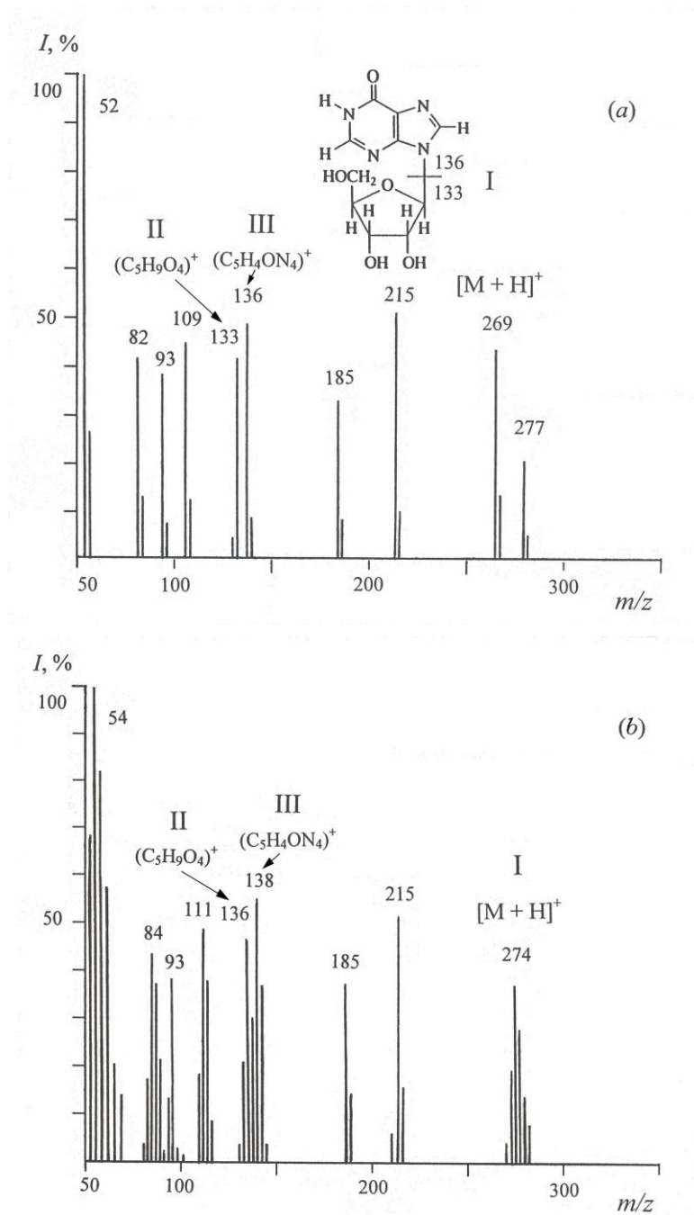
Figure 4. FAB mass spectra of inosine (glycerol as a matrix) under different experimental conditions: (a) – natural inosine; (b) – [ 2 H]inosine isolated from HW medium (scanning interval at m/z 50–350; major peaks with a relative intensity of 100% at m/z 52 and m/z 54; ionization conditions: cesium source; accelerating voltage, 5 kV; ion current, 0.6–0.8 mA; resolution, 7500 arbitrary units): I – relative intensity of peaks (%); (I) – inosine; (II) – ribose fragment; (III) – hypoxanthine fragment.
