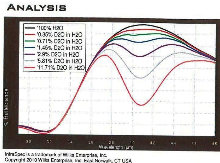
Figure 4. The typical IR-spectra of water with varying content of deuterium
