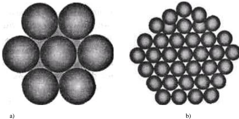
Figure 5. The sphere (a) and the pentagonal (b) packing of balls representing \text{H}_2\text{O} molecules in clusters.
