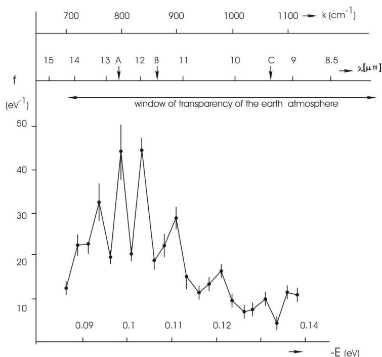
Figure 5: NES-spectrum of deionized water (chemical purity – 99.99 %; pH – 6.5–7.5; total mineralization – 200 mg/l; electric conductivity – 10 \mu S/cm). The horizontal axis shows the energy of the H...O hydrogen bonds in the associates – E (eV). The vertical axis – energy distribution function – f ( eV^{-1} ). k – the vibration frequency of the H–O–H atoms ( cm^{-1} ); \lambda – wavelength ( \mu m ).
