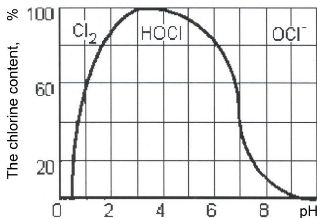
Figure 4: Content (%) of various forms of chlorine (Cl 2 , HOCl, OCl - ) in the electrochemically activated water depending on the pH value
