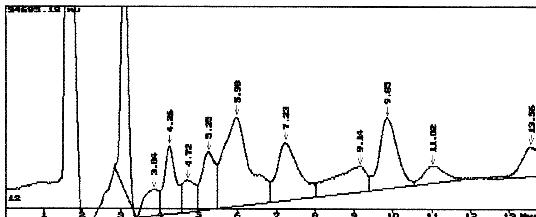
Figure 3. HPLC-chromatograms of intracellular carbohydrates obtained from protonated (a) and deuterated (b) cells of B. subtilis on the maximally deuterated D 2 O-medium: Knauer Smartline chromatograph (250×10 mm) (“Knauer”, Germany); stationary phase: Ultrasorb CN; 10 µm; mobile phase: acetonitrile–water (75:25, % (w/w); the input rate: 0.6 ml/min
