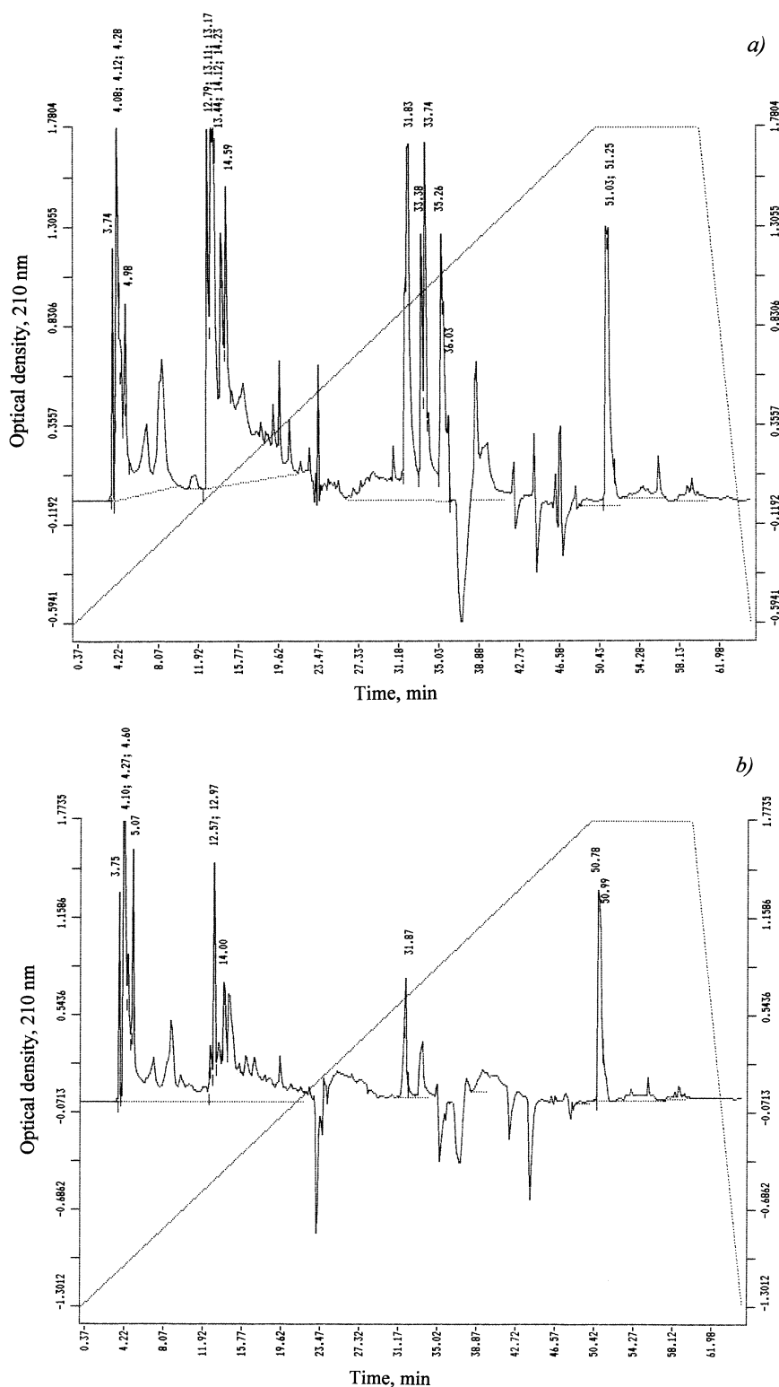
Figure 1. HPLC-chromatograms of fatty acids obtained from protonated (a) and deuterated (b) cells B. subtilis on the maximally deuterated D 2 O-medium. The peaks on chromatograms with retention time 3.75 min (instead of 3.74 min in the control), 4.10; 4.27; 4.60 (instead of 4.08; 4.12; 4.28 in the control), 5.07 (instead of 4.98 in control) 12.57; 12.97 (instead of 12.79; 13.11; 13.17 in control) 14.00 (instead of 14.59 in the control), 31.87 (instead of 31.83 in the control); 33.38; 33.74; 33.26; 36.03; 50.78; 50.99 (instead of 51.03; 51.25 for control) correspond to individual intracellular fatty acids
