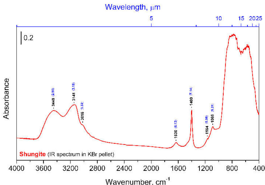
Figure 4. IR-spectra of shungite in KBr pellet (spectral range: average IR – 370–7800 \text{cm}^{-1} ; visible – 2500–8000 \text{cm}^{-1} ; the permission – 0,5 \text{cm}^{-1} ; accuracy of wave number – 0,1 \text{cm}^{-1} on 2000 \text{cm}^{-1} )
