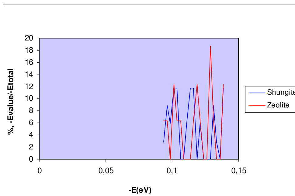
Figure 5. The distribution [% \cdot(-E_{\text{value}})/(-E_{\text{total value}}) ] of water molecules in water solution of shungite/zeolite according to energies of hydrogen bonds (-E value ) to the total result of hydrogen bonds energy
