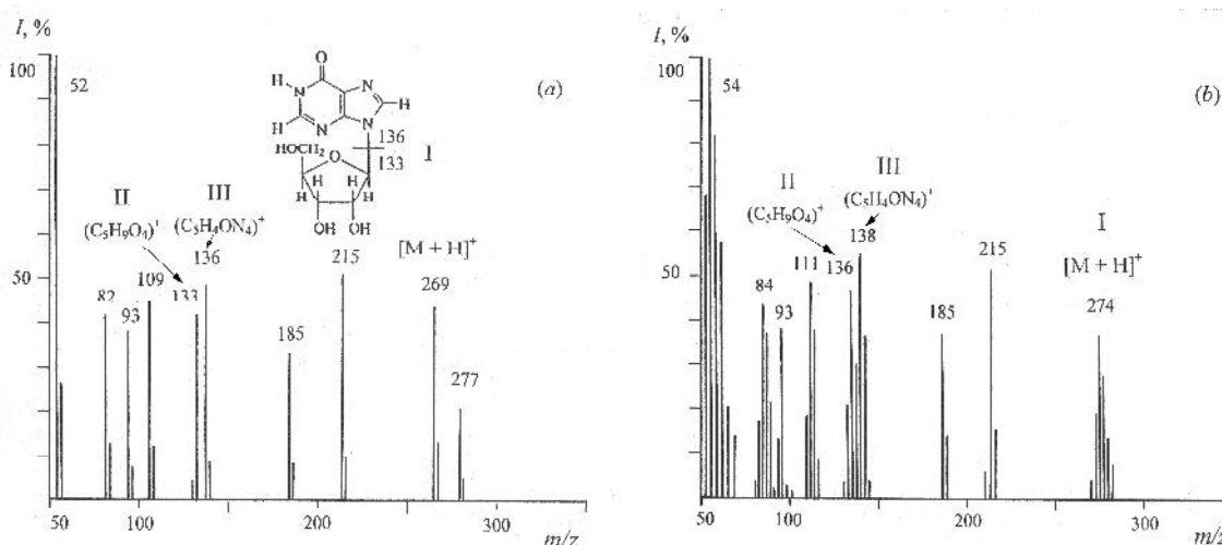
Figure 6: FAB mass spectra of inosine (glycerol as a matrix) under different experimental conditions: (a) – natural inosine; (b) – [^2\text{H}] inosine isolated from HW medium (scanning interval at m/z 50–350; major peaks with a relative intensity of 100% at m/z 52 and m/z 54; ionization conditions: cesium source; accelerating voltage, 5 kV; ion current, 0.6–0.8 mA; resolution, 7500 arbitrary units): I – relative intensity of peaks (%); (I) – inosine; (II) – ribose fragment; (III) – hypoxanthine fragment.
