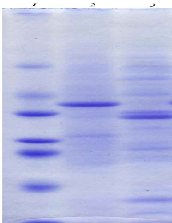
Figure 13: Electrophoregrams of proteins isolated from hydrolysates of total biomass of B. subtilis : 1 – a standard set of proteins; 2 – a sample obtained from protonated medium; 3 – a sample obtained from \text{D}_2\text{O} -medium
