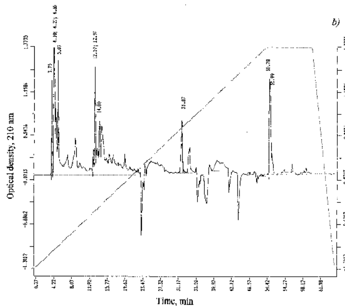
Figure 10: HPLC-chromatograms of fatty acids obtained from protonated (a) and deuterated (b) cells of B. subtilis on the maximally deuterated ^2\text{H}_2\text{O} -medium: Beckman Gold System (Beckman, USA) chromatograph (4.6x250 mm); stationary phase: Ultrasphere ODS, 5 \mu\text{m} ; mobile phase: linear gradient 5 mM \text{KH}_2\text{PO}_4 -acetonitrile (shown in phantom), elution rate: 0.5 ml/min, detection at \lambda = 210 nm. The peaks with retention time 3.75 min (instead of 3.74 minutes in the control), 4.10; 4.27; 4.60 (instead of 4.08; 4.12; 4.28 in the control), 5.07 (instead of 4.98 in control) 12.57; 12.97 (instead of 12.79; 13.11; 13.17 in control) 14.00 (instead of 14.59 in the control), 31.87 (instead of 31.83 in the control); 33.38; 33.74; 33.26; 36.03; 50.78; 50.99 (instead of 51.03; 51.25 for control) correspond to individual intracellular fatty acids
