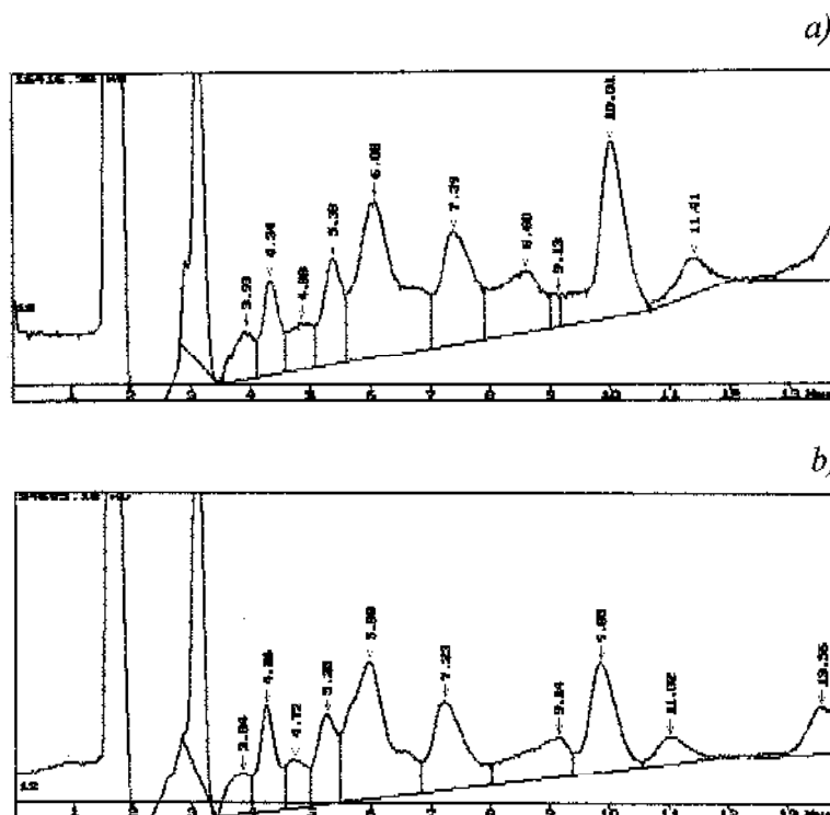
Figure 12: HPLC-chromatograms of intracellular carbohydrates obtained from protonated (a) and deuterated (b) cells of B. subtilis on the maximally deuterated 2 H 2 O-medium: Knauer Smartline chromatograph (250×10 mm) (“Knauer”, Germany); stationary phase: Ultrasorb CN; 10 μm; mobile phase: acetonitrile–water (75:25, % (w/w); the input rate: 0.6 ml/min
