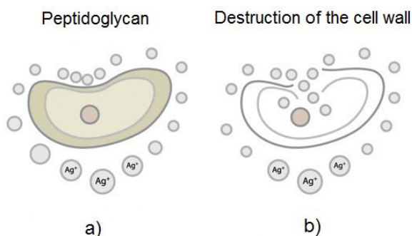
Figure 2: Schematic representation of the interaction of \text{Ag}^+ ions with the microbial cell: a) – the interaction of \text{Ag}^+ ions with the membrane protein peptidoglycan; b) – the process of destruction by \text{Ag}^+ ions the cell wall and further penetration into the microbial cell
