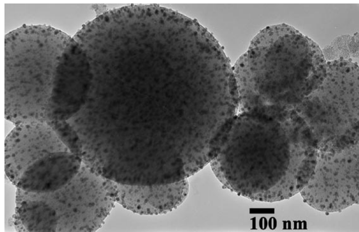
Figure 3: Electron micrographs of micro silver nanoparticles fixed on the surface of spherical particles of the mesoporous aluminosilicate \text{Na}_2\text{O}\cdot\text{Al}_2\text{O}_3\cdot n\text{SiO}_2\cdot m\text{H}_2\text{O} , where n = 1-10 , m = 1-2 (Rybaltoivskiy et al. , 2015)
