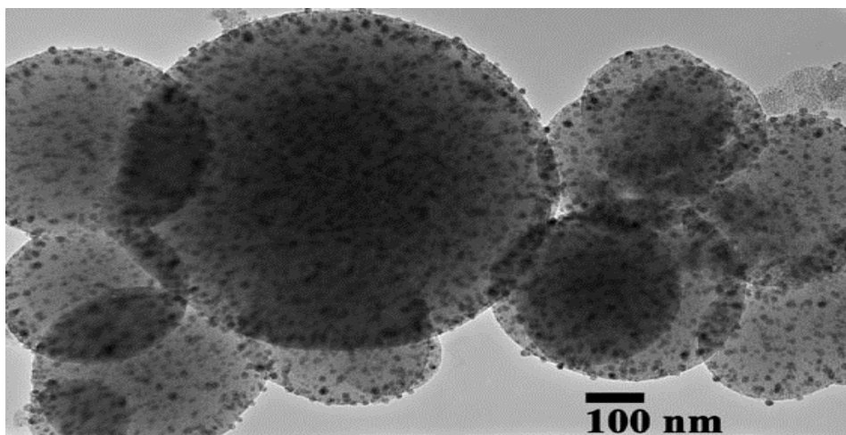
Figure 2. Electron micrographs of micro silver nanoparticles fixed on the surface of spherical particles of the mesoporous aluminosilicate \text{Na}_2\text{O} \cdot \text{Al}_2\text{O}_3 \cdot n\text{SiO}_2 \cdot m\text{H}_2\text{O} , where n = 1-10 , m = 1-2 (Khaydarov et al. , 2009)
