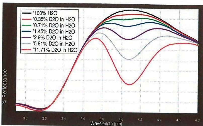
Figure 5: The typical IR-spectra of water with varying content of deuterium
