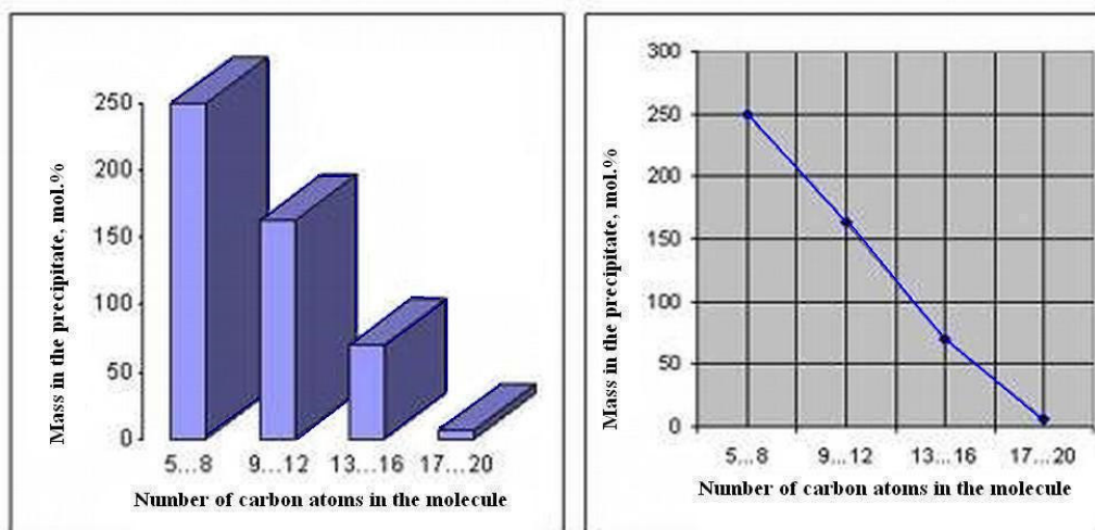
Figure 7: Distribution of carbon compounds obtained in the experiments of S. Miller, mass and number of carbon atoms in the molecule (diagrams constructed by the authors according to the S. Miller experiments)
