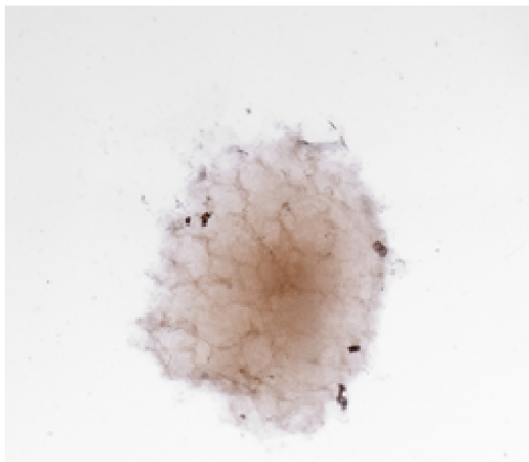
Figure 8: The organized structure in water sample subjected to the temperature +100 °C in the electric field of high voltage and frequency. The material of the electrode – hostafan; electric voltage – 15 kV, electric impulse duration – 10 μs; electric current frequency – 15 kHz.
