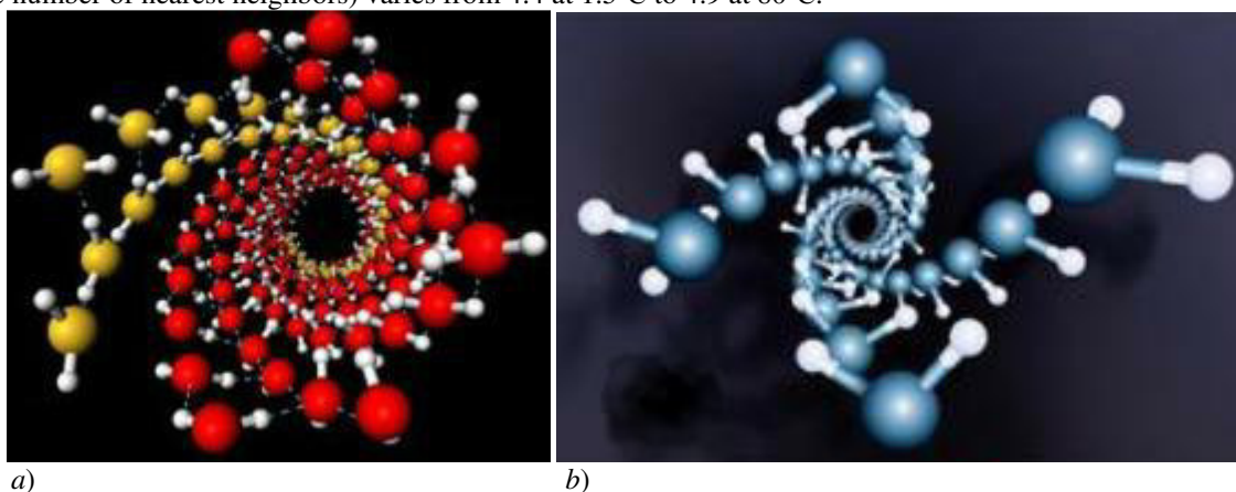
Figure 6: Structures of water crystals in carbon nanotubes according to computer simulations (Bai et al. , 2006) (diameter of nanotubes 1.35–1.90 nm; pressure 10–40000 atm; temperature -23°C): a) – a general view of the crystal structure of water in nanotubes, b) – the inner wall of the structure of water.
