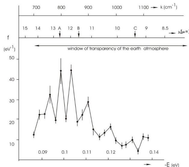
Figure 3: Non-equilibrium (NES) spectrum of water; \lambda – wavelength; k – wave number The study of the IR spectrum of water in the composition of physiologic fluids (urine, blood, serum)
