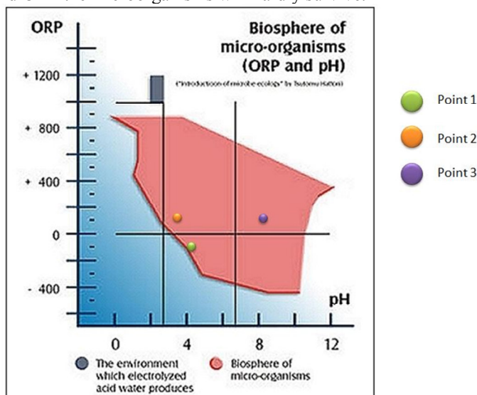
Figure 3. The dependence between acidity and basicity (pH) of solutions and the ORP on the biosphere of micro-organisms (point 1; VITA Intense), (point 2; BOOST), point 3; ZEOLITH detox).
