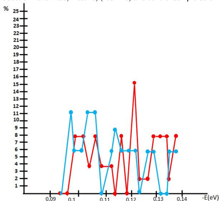
Fig. 3. Mathematical model (Ignatov, Mosin, 2013) of 1% water solution of ZEOLITH Creme (product of LavaVitae, Austria).
