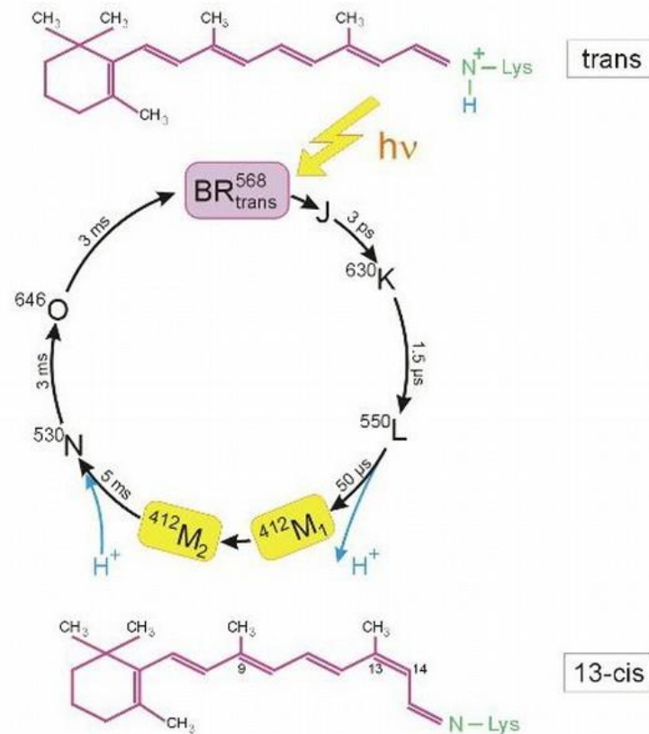
Figure 6. Photocycle scheme of BR (aqueous solution, pH = 7.2, t = 20 °C). Latin numbers J, K, L, M, N, O denote the spectral intermediates of BR. M 1 and M 2 represent spectral intermediants of meta - bacteriorhodopsin with the protonated and deprotonated aldimine bond. The superscripts correspond to the position of the absorption maximum of the photocycle intermediates (nm)
