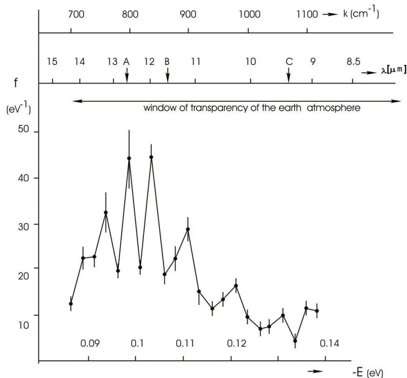
Fig. 4. Non-equilibrium energy spectrum (NES) of water as a result of measurement for 1 year: \lambda – wavelength, k – wave number.
