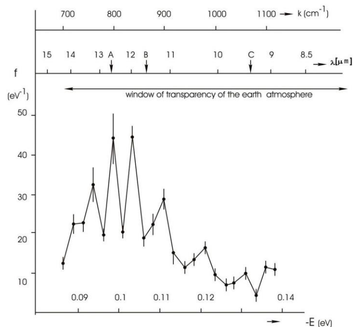
Fig. 5. Non-equilibrium energy spectrum (NES) of water as a result of measurement for 1 year: \lambda – wavelength, k – wave number.
