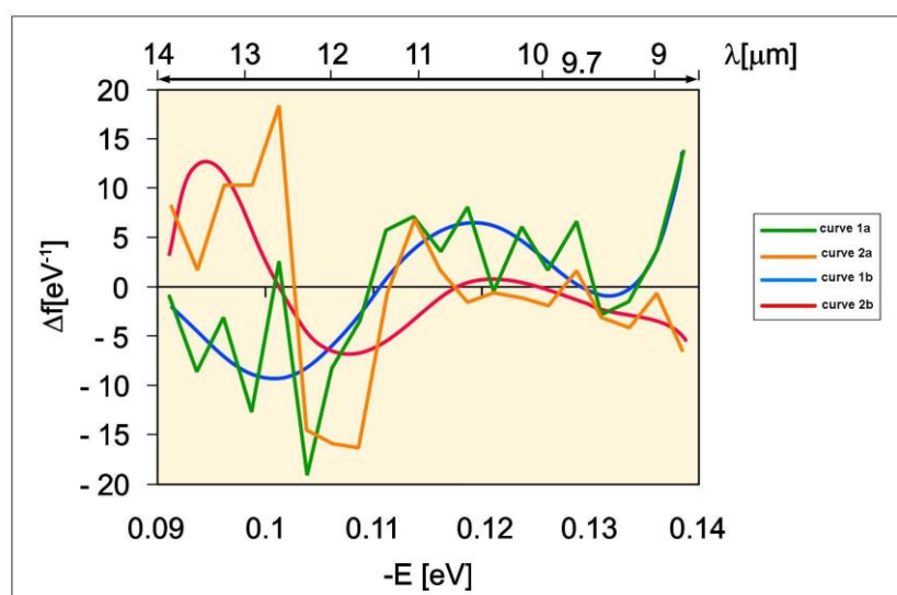
Fig. 6. Differential non-equilibrium energy spectrum (DNES) reflecting the heat exchange of the human body with surrounding environment.
