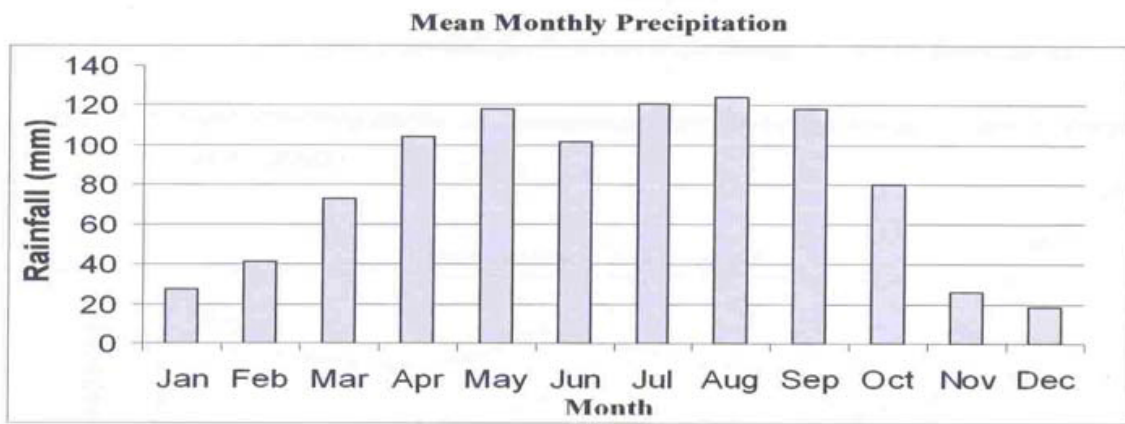
Fig.1 Mean Monthly precipitation of Hawassa
