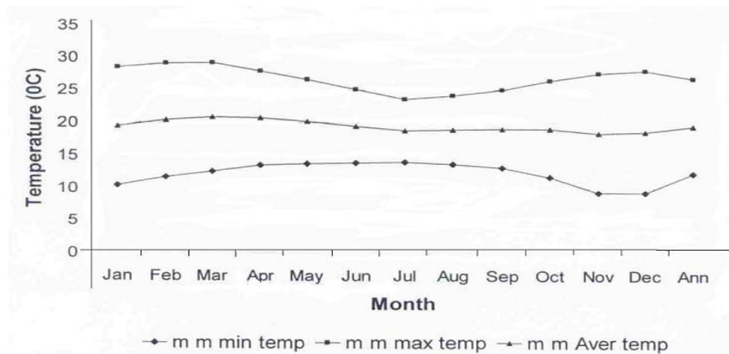
Fig.2 Mean monthly minimum, maximum and average temperature at Hawassa
