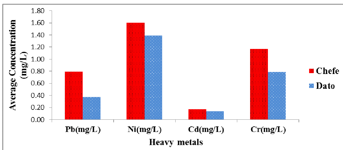
Fig 5. Distribution of concentration of Pb, Ni, Cd and Cr in fresh cow's milk from Chafe and Dato
