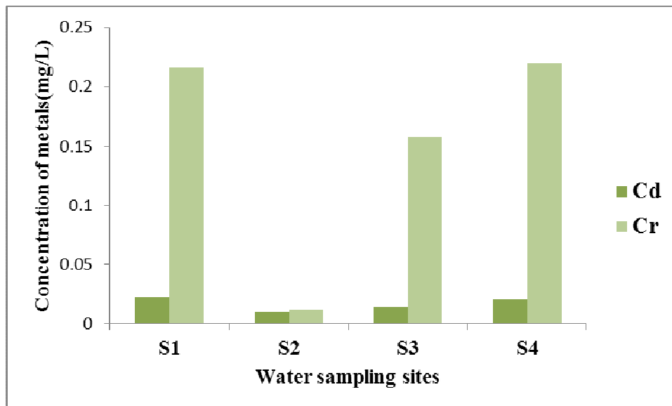
Fig 4. Distribution of Cadmium and Chromium concentrations in the Textile Factory treatment ponds water and Tikur-Wuha River
