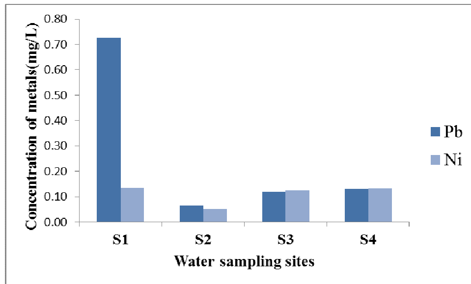
Fig 3. Distribution of concentration of Lead and Nickel in the Textile Factory treatment ponds water and Tikur-Wuha River
