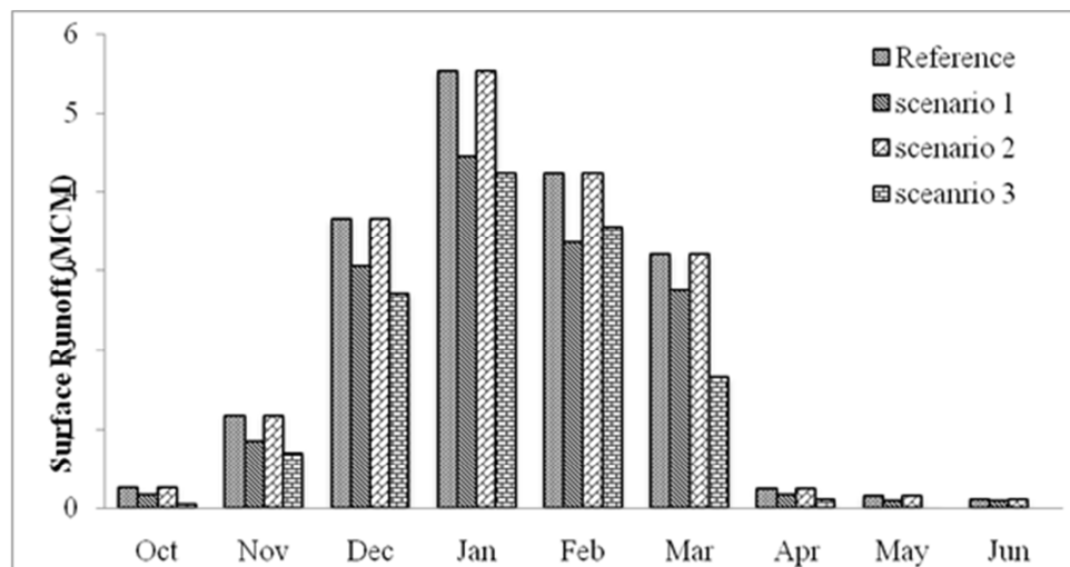
Figure 9: Projected Runoff over the Period (2014–2050) on Monthly Basis under Different Climate Change Scenarios
