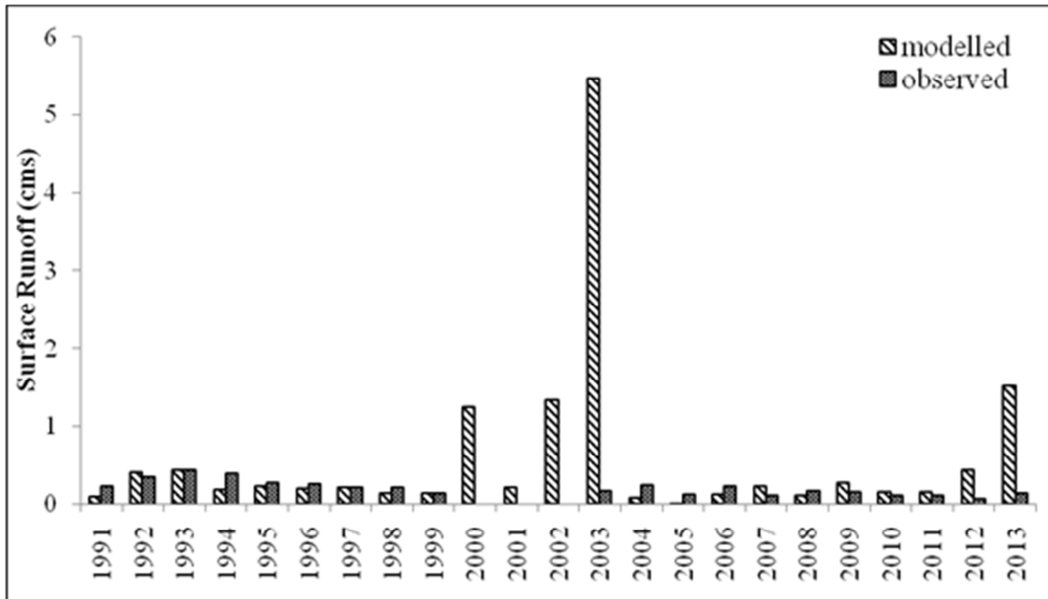
Figure 7: Simulated Surface Runoff (calibrated) versus Observed Streamflow Values for the Reference Scenario With regards to the model performance criterion, a scatter plot of annual modeled (calibrated) versus observed runoff using SPSS statistical software is shown in Figure 8. Even after final calibration has been done, the simulated runoff was over-estimated in the years 2000, 2002, 2003 and 2013; the extreme values were excluded when measuring the modeling performance. The correlation between the scattered dots using SPSS found to be 0.612; this means that the simulated and observed runoff values are well correlated to each other.
