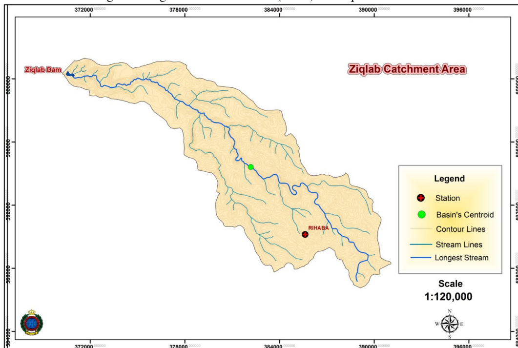
Figure 3: Ziqlab catchment area derived from DEM with the main parameters and gauging stations
