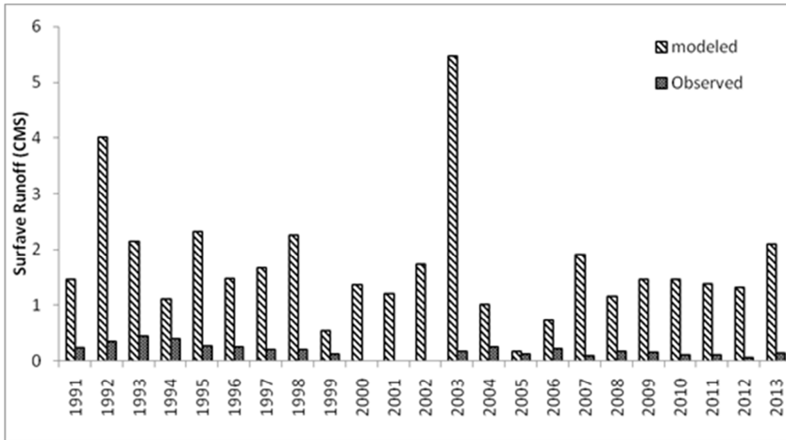
Figure 6: Simulated Surface Runoff (un-calibrated) versus Observed Streamflow Values for the Reference Scenario
