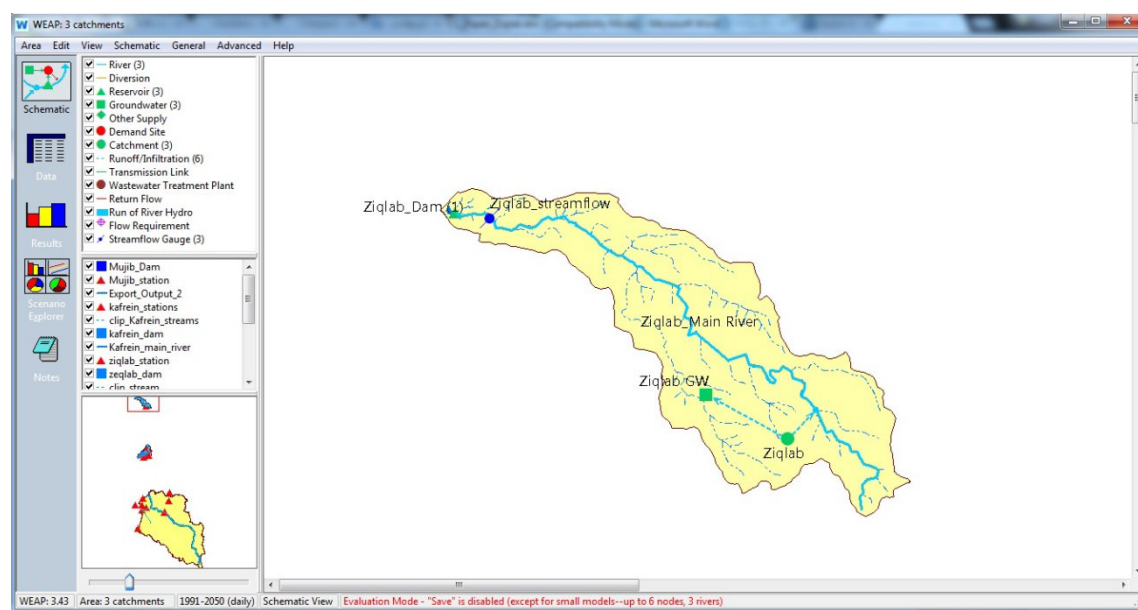
Figure 4: Schematic of the WEAP model for Ziqlab Dam catchment
