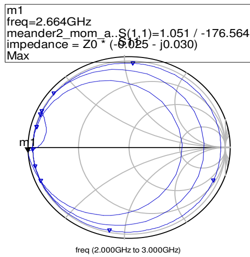
Figure 2: Simulated input impedance of Meander Microstrip patch
