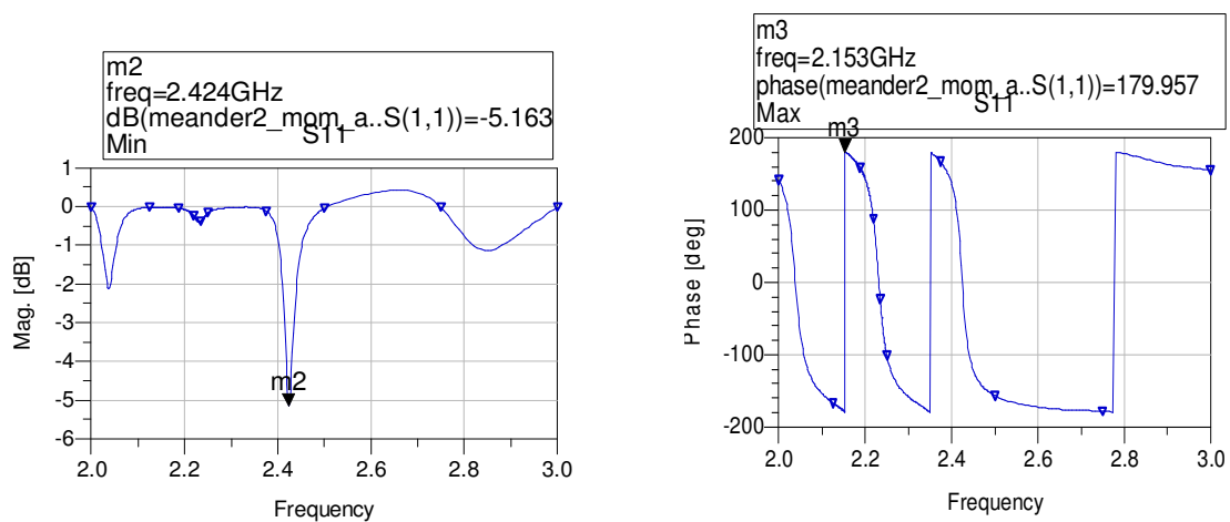
Figure 1: Output Return Loss and input return loss
