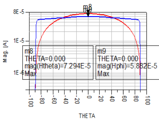
Figure 5: 2D Magnetic Field Radiation pattern
