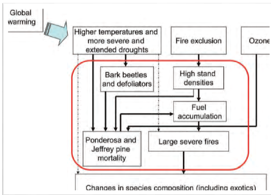
Figure 3: the effect of global warming on insect and forest fire
