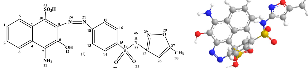
Figure (1): The ( Z )-4-amino-3-hydroxy-2-((4-( N -(5-methylisoxazol-3-yl)sulfamoyl)phenyl)di azenyl) naphthalene-1-sulfonic acid (1).
