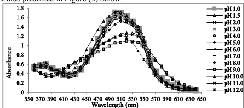
Figure 2: The pH effect of azodye (1).
