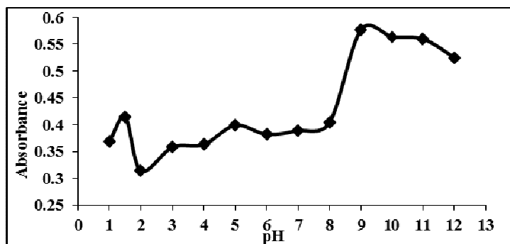
Figure 3: Absorbance-pH effect of azodye (1) at \lambda_{420} nm.
