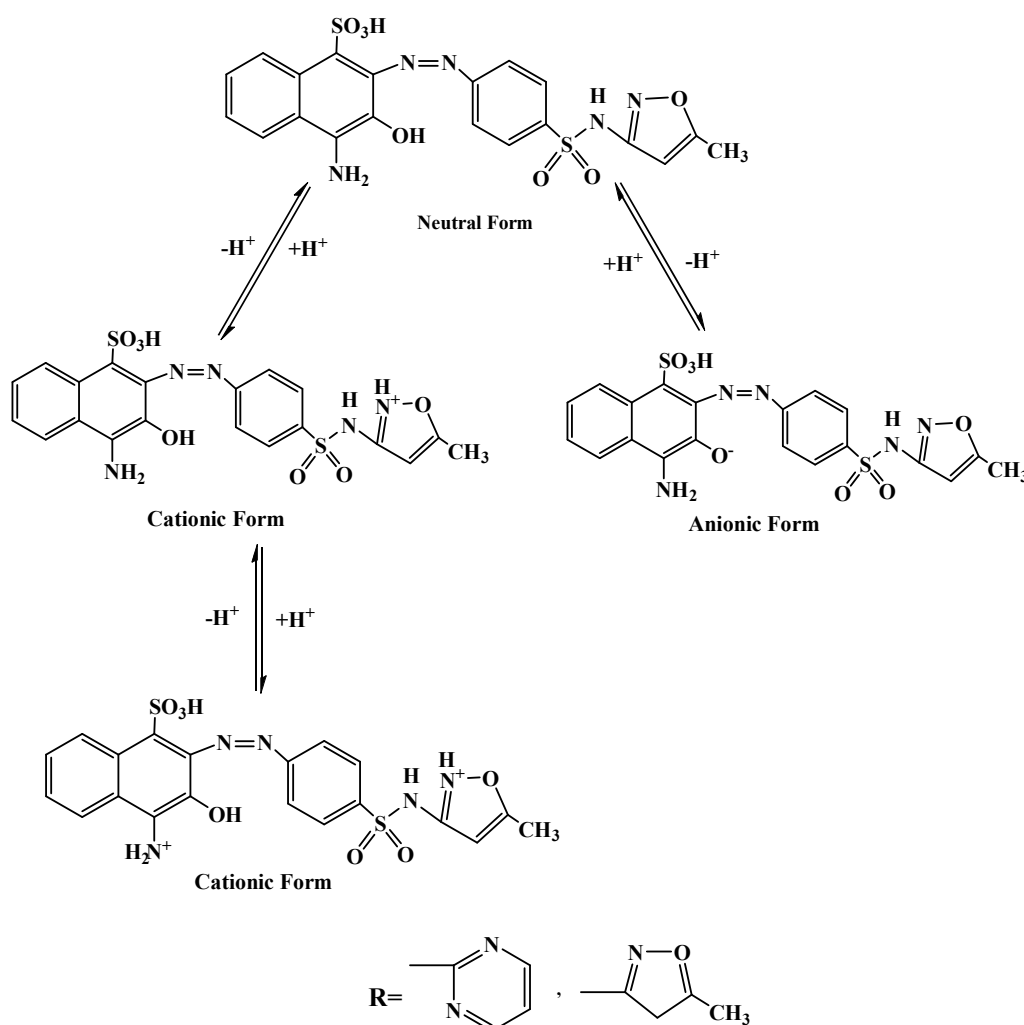
Scheme (1): The suggested ionization of azodye (1) in acidic and basic medium.
